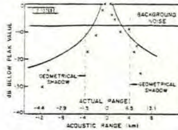
Fig. 13. Detection data for A-7 (altitude = 1020 m, 0 dB = 88 dBa).
