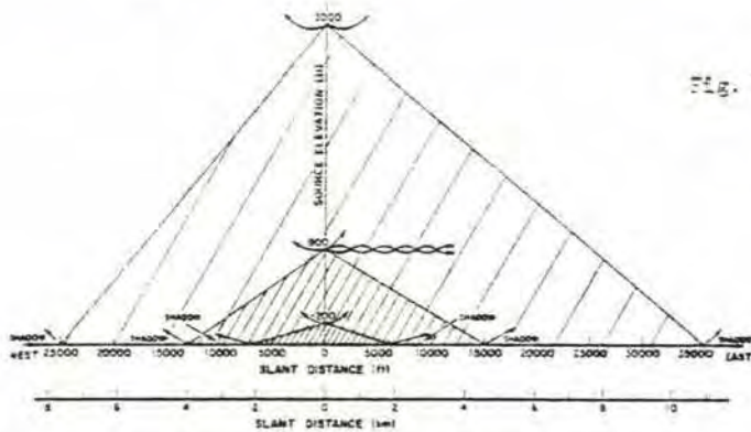
Fig. 12. Detection data for A-7 (altitude = 450 m, 0 dB = 87 dBa).
