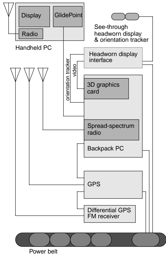
Figure 6. Hardware design of our prototype campus information system.
