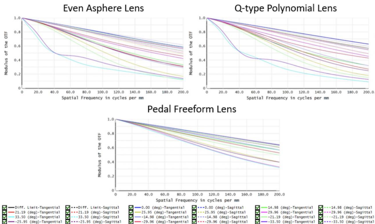
Figure 3.27. MTF plots under 5 \mu\text{m} decenter of surface 7 in Y direction for the even asphere lens, the Q- type polmyomial lens and the pedal freeform lens
