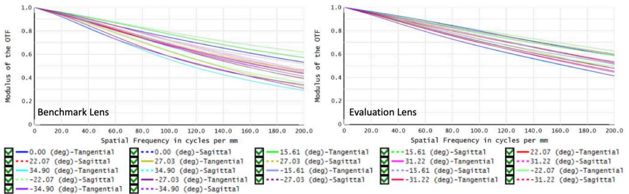
Figure 3.13. MTF plots of benchmark lens (left) and evaluation lens (right) under 5 \mu\text{m} decenter of surface 10 in Y direction
