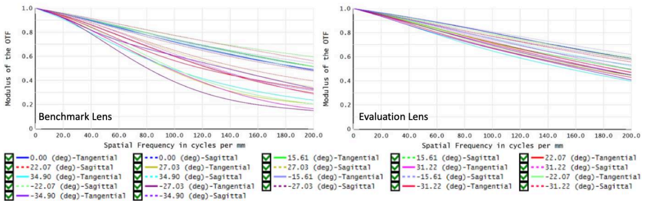
Figure 3.14. MTF plots of benchmark lens (left) and evaluation lens (right) under 5 \mu\text{m} decenter of element 4 in Y direction
