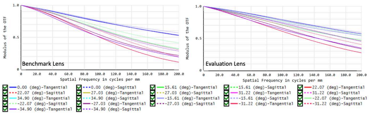
Figure 3.16. MTF plots of benchmark lens (left) and evaluation lens (right) under 5 μm decenter of surface 7 in X direction
