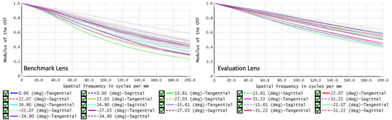
Figure 3.12. MTF plots of benchmark lens (left) and evaluation lens (right) under 5 \mu\text{m} decenter of surface 9 in Y direction
