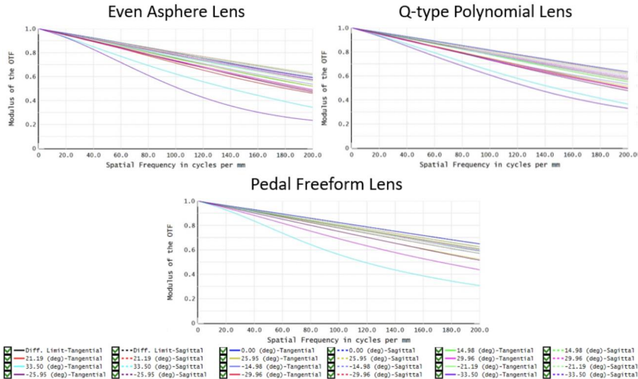
Figure 3.28. MTF plots under 5 \mu\text{m} decenter of surface 8 in Y direction for the even asphere lens, the Q- type polmyomial lens and the pedal freeform lens
