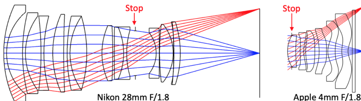
Figure 3.2. Layout comparison between the Nikon 28mm conventional camera lens and Apple 4mm miniature camera lens
