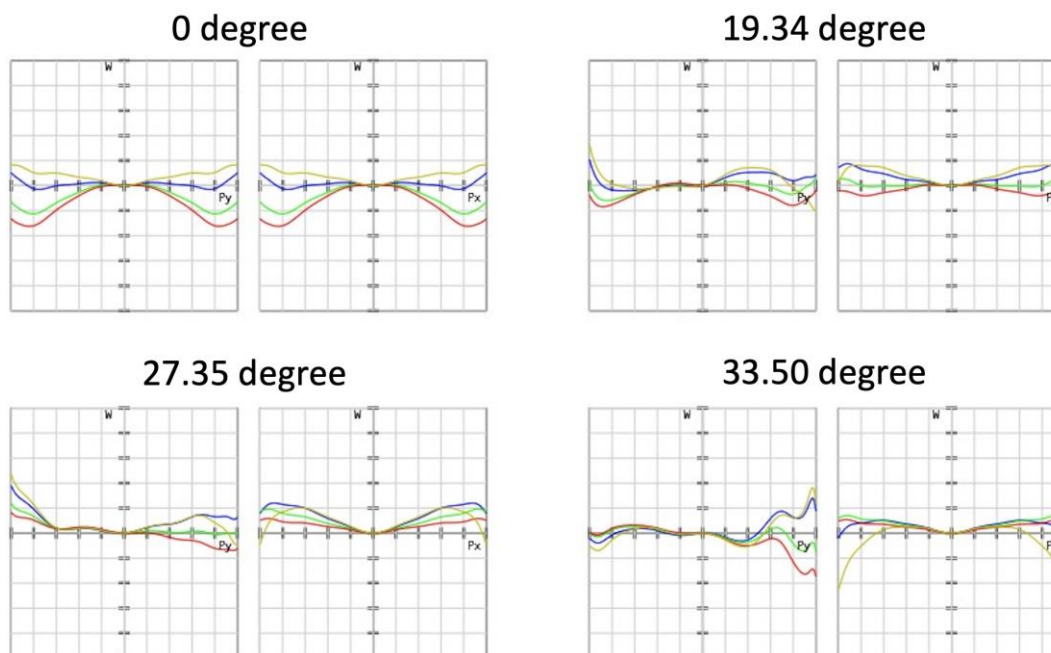
Figure 3.24. Nominal OPD plots of the Q-type polynomial lens
