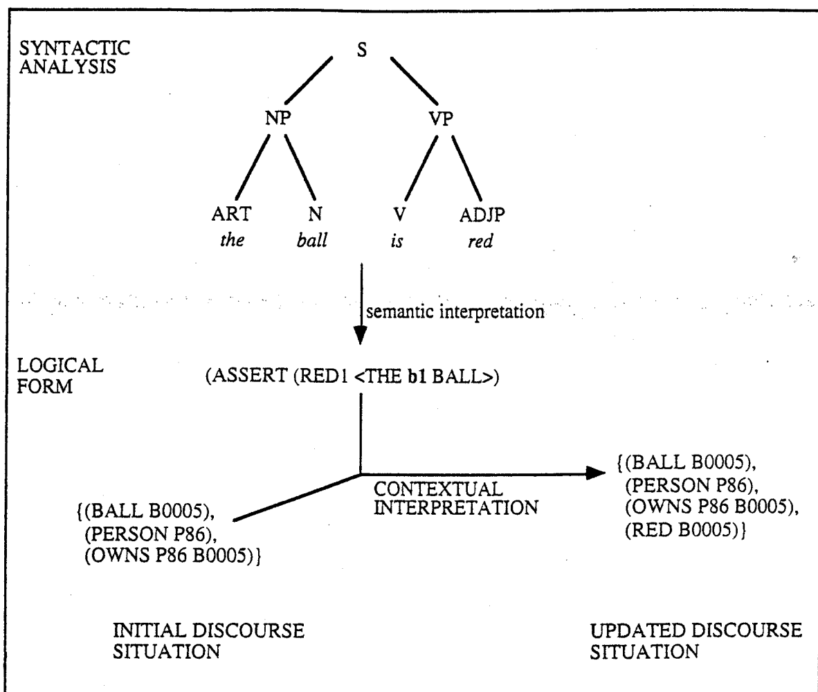
Figure 8.2 Logical form as a function
