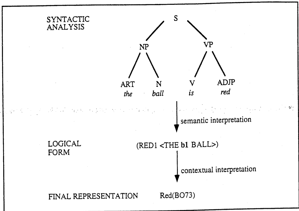
Figure 8.1 Logical form as an intermediate representation
