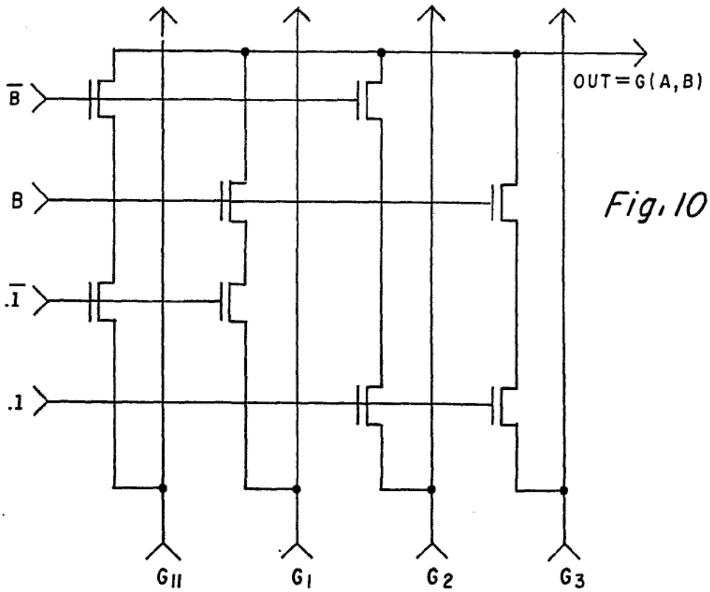
FUNCTIONAL BLOCK IN ALU
