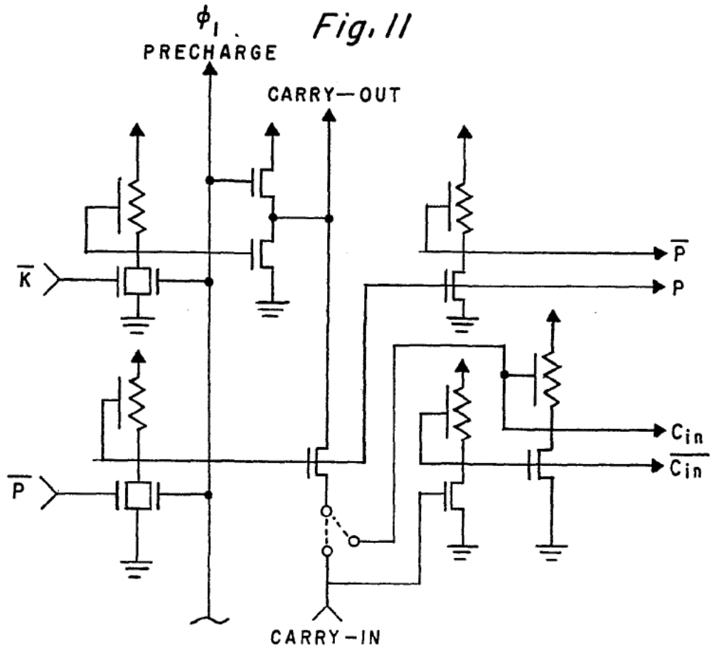
FUNCTIONAL BLOCK IN ALU
