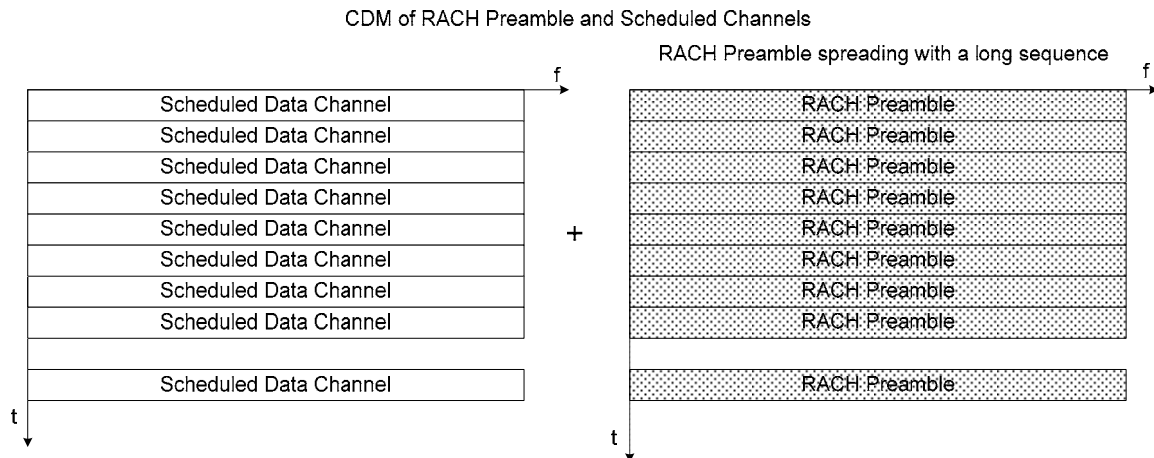
Figure 2 CDM of Scheduled Channels and RACH Preamble
