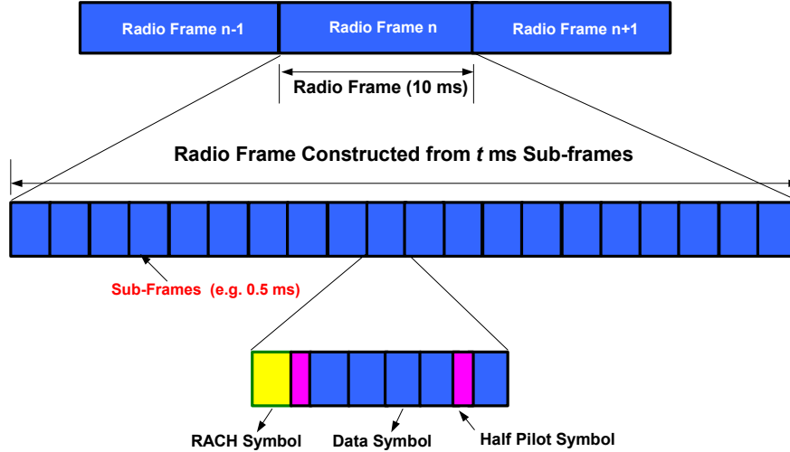
Figure 3. TDM/FDM RACH Structure
