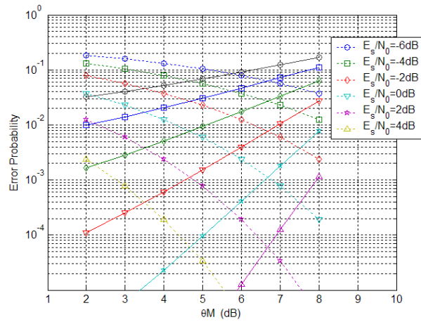
Figure 4 Detection Error and False Alarm Probabilities of TDM-RACH over AWGN Channel.
