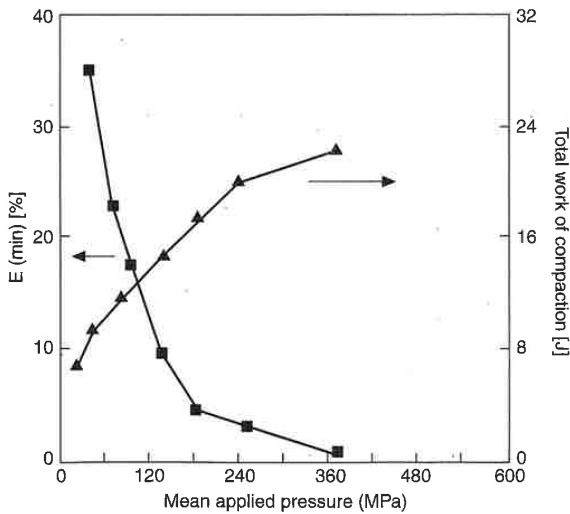
Fig. 2: Total work of compaction.
