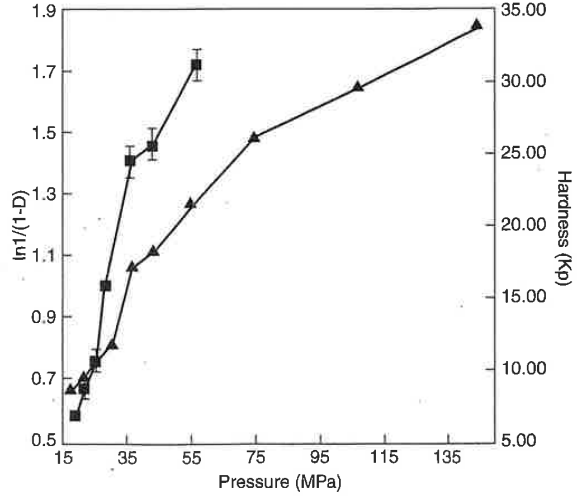
Fig. 3: Heckel plot for microcrystalline cellulose.
