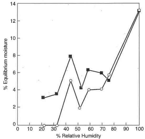
Fig. 4: Sorption-desorption isotherm for microcrystalline cellulose.
