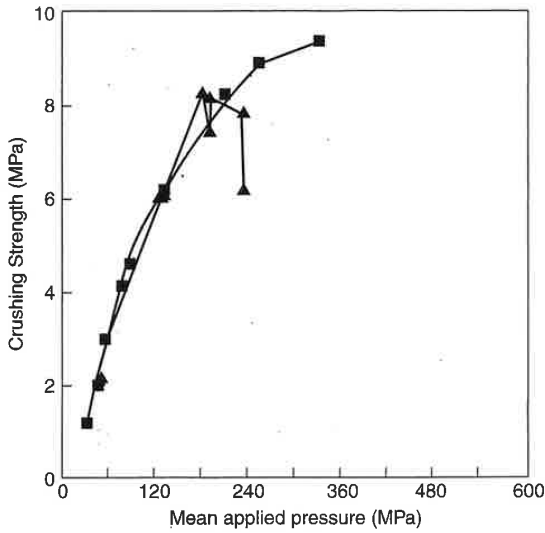
Fig. 1: Crushing strength.
