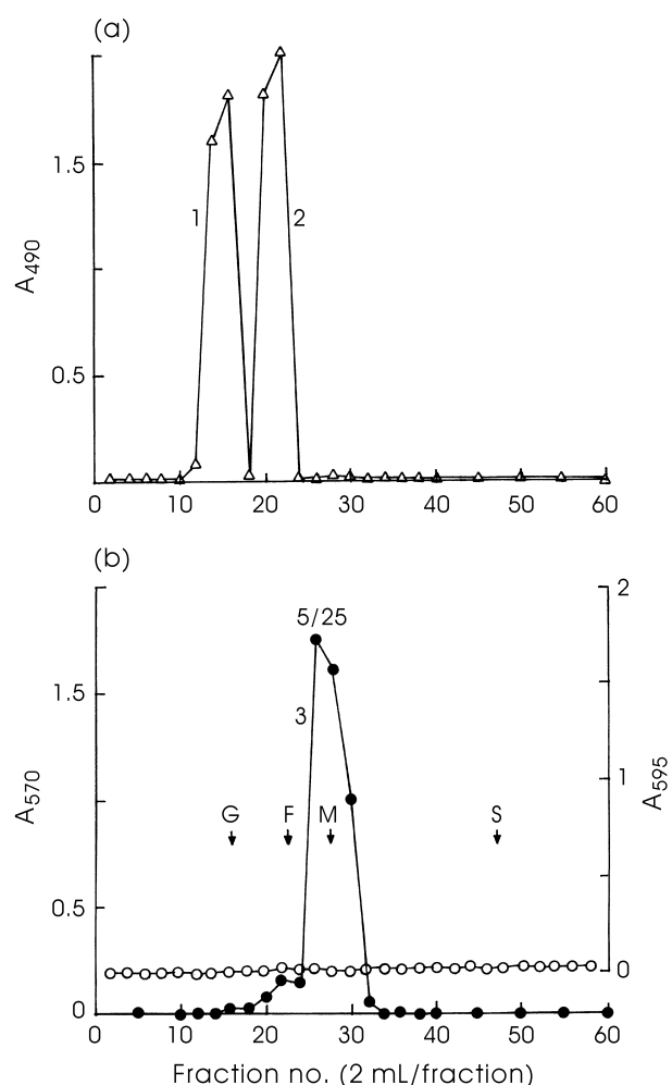
Fig. 2 \text{Ca}^{2+} ion-moderated cation-exchange chromatography of Agaricus bisporus 3K-filtrate (0.5 mL, 10x concentrated) on a Dowex 50 W column (1 x 60 cm, 8% cross-linked, 200–400 dry mesh). The eluent was water; the flow rate was 15 mL/h. (a) Detection by phenol-sulfuric acid ( -\triangle- ). (b) Polyol detection, A_{570} ( -\bullet- ); Bradford's protein assay, A_{595} ( -\circ- ). The numbers above peak 3 indicate wheal/flare diameter (mm) produced by the peak fractions 26 and 28. Other fractions tested (6, 16, 22, 24, 30 and 32) did not produce a wheal/flare reaction. Arrows indicate elution positions of standards under identical conditions: D-glucose (G), D-fructose (F), D-mannitol (M), sorbitol (S).
