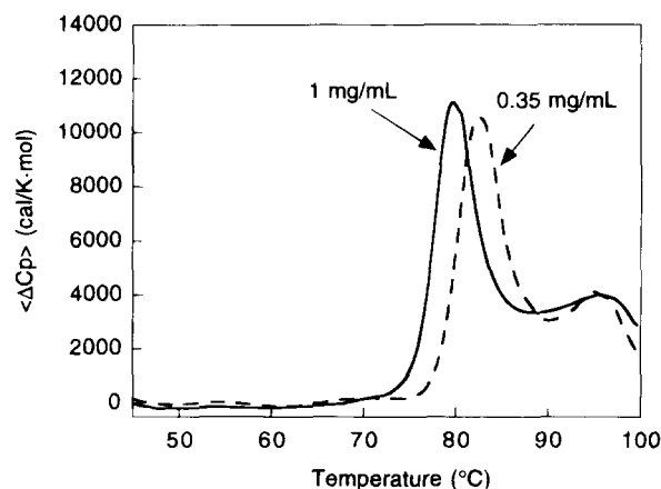
Fig. 5. Excess heat capacity of rhGH at pH 7.5.
