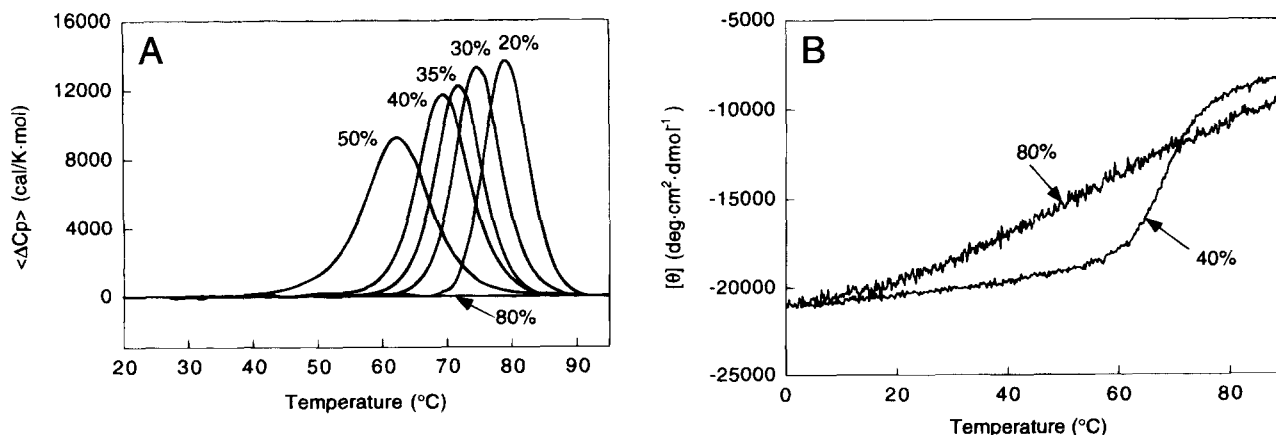
Fig. 8. A: Excess heat capacity of rhGH at pH 7.5 in different propylene glycol concentrations. B: Temperature-induced unfolding of rhGH at pH 7.5 in 40 and 80% propylene glycol monitored by CD at 222 nm.
