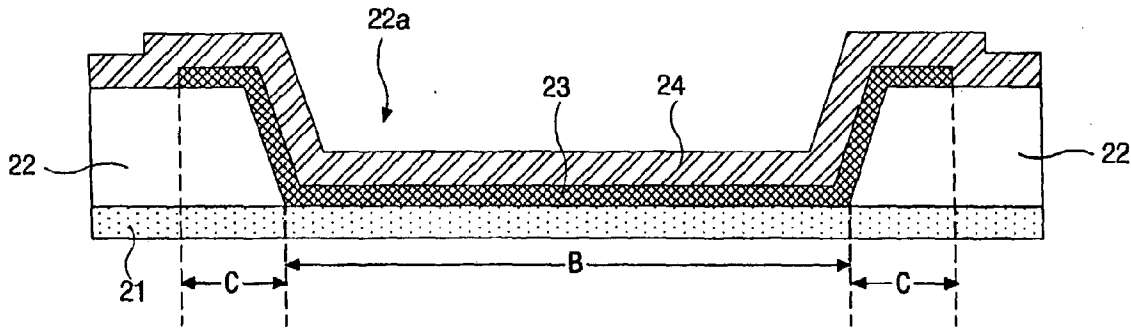
FIG. 3 Related Art
