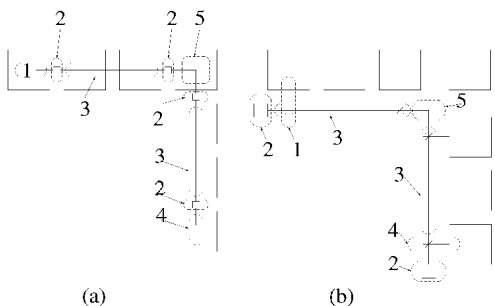
Fig. 17. Length 6 net connection with a bend in new fabric (a) and in baseline fabric (b). The numbers correspond to (1) output segment, (2) routing point/ switching point, (3) interconnect segment, (4) input segment, and (5) signal bend.
