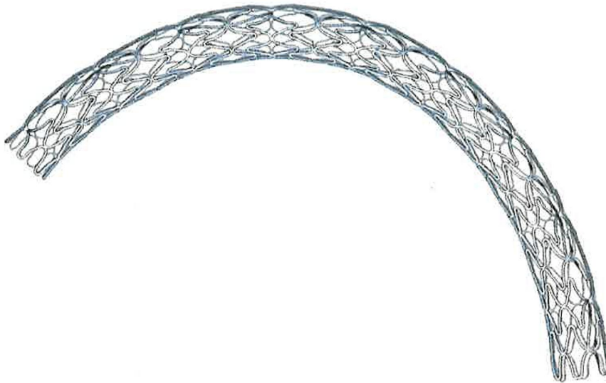
Figure 33.1: Tsunami – conformability.
