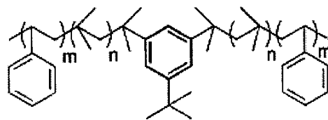
Figure 2. The Chemical Structure of SIBS [poly(styrene-b-isobutylene-b-styrene)]
