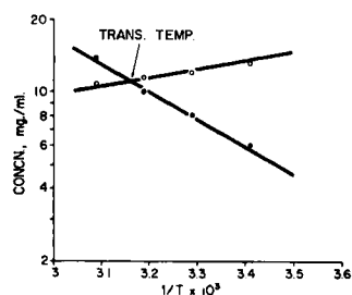
Fig. 3—The van't Hoff-type plot for the anhydrous and
