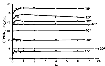
Fig. 1—The dissolution behavior of anhydrous and trihydrate crystalline forms of ampicillin in water at
