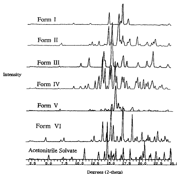
Fig. 3. Zanoterone XRPD patterns for forms I–VI and acetonitrile solvate. Scinta XDS system; 5° (2 \theta )/min.
