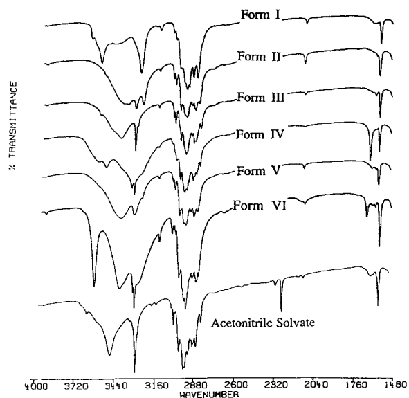
Fig. 2. Zanoterone FTIR data for forms I–VI and acetonitrile solvate. Nicolet 730 FTIR; 1% potassium bromide pellet.
