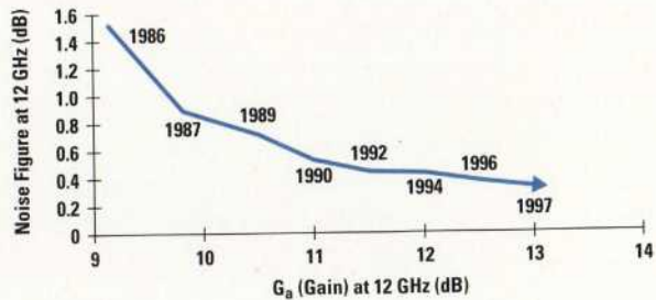
Figure 2 GaAs transistor performance for DBS applications.
