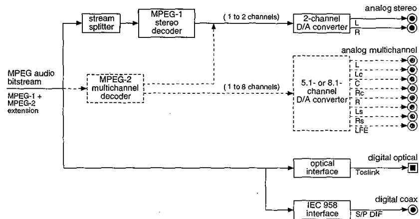
Figure 4.39 MPEG-2 audio block diagram.
