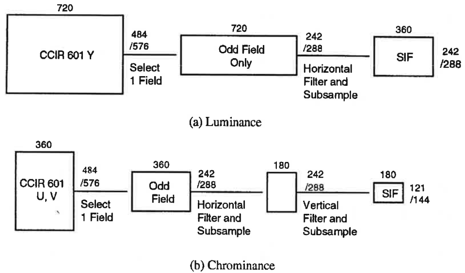
Figure D.12 -- Conversion from CCIR 601 into SIF
