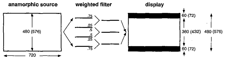
Figure 4.33 Letterbox conversion.
