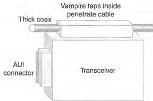
Figure 7-4 A 10Base5 network uses an external transceiver, connected to thick coax by vampire taps.
