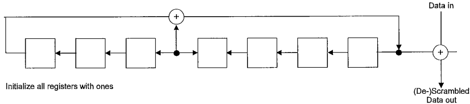
Figure 71—Frame synchronous scrambler/descrambler
