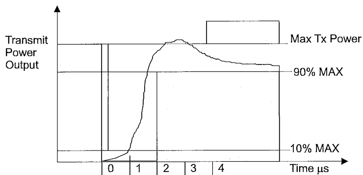
Figure 97—Transmit power-on ramp
