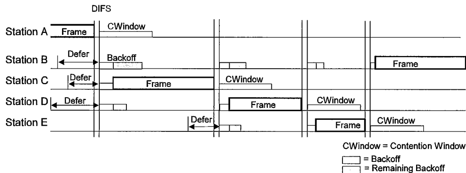
Figure 52—Backoff procedure
