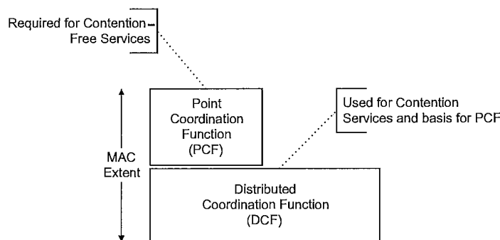
Figure 47—MAC architecture
