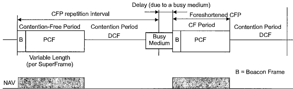
Figure 59—CFP/CP alternation
