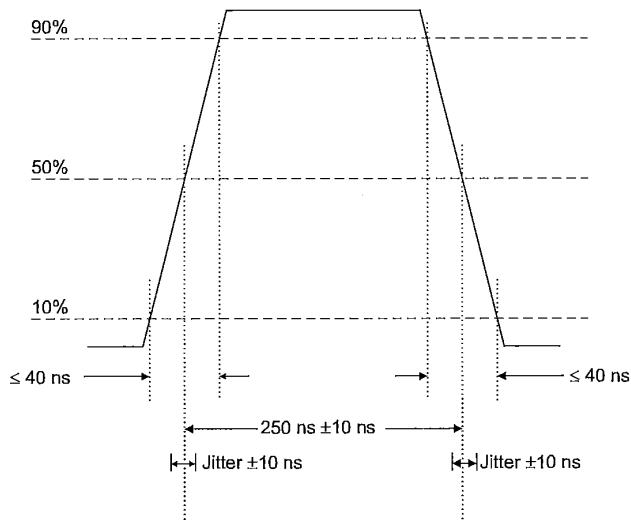
Figure 102—Basic pulse shape
