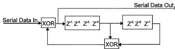
Figure 89—Data scrambler
