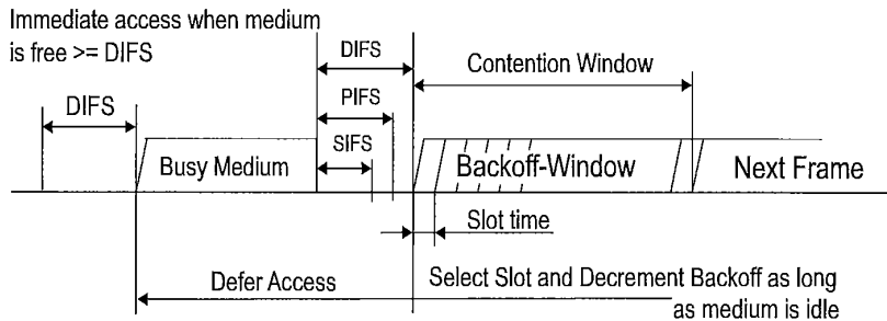
Figure 51—Basic access method
