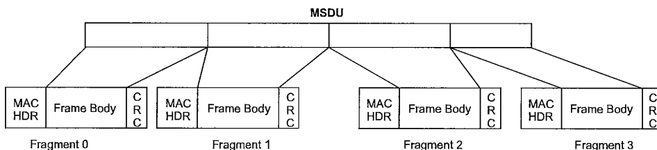
Figure 48—Fragmentation
