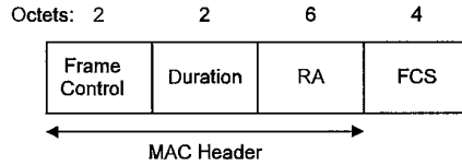
Figure 17—CTS frame
