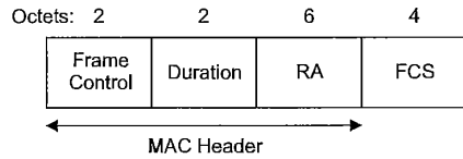
Figure 18—ACK frame
