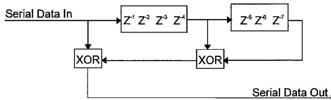
Figure 90—Data descrambler
