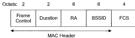
Figure 20—CF-End frame
