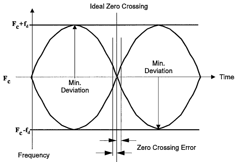
Figure 84—Transmit modulation mask
