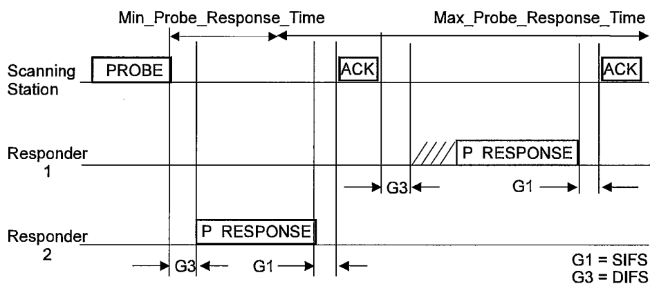
Figure 66—Probe response
