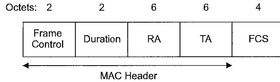
Figure 16—RTS frame
