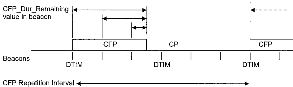
Figure 60—Beacons and CFPs
