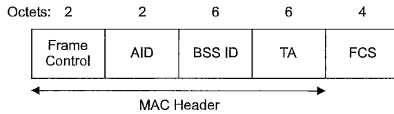
Figure 19—PS-Poll frame
