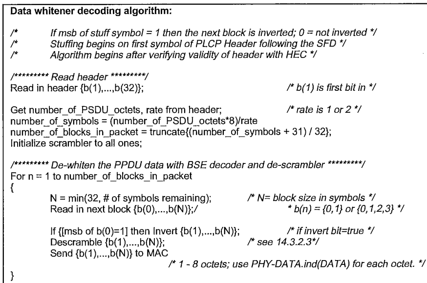
Figure 80—Data whitener decoding procedure
