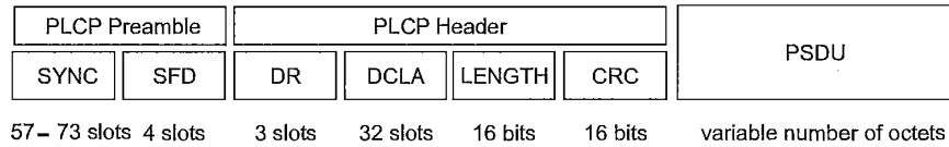
Figure 101—PLCPDU frame format
