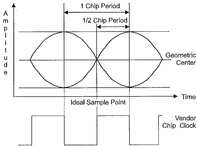
Figure 100—Chip clock alignment with baseband eye pattern
