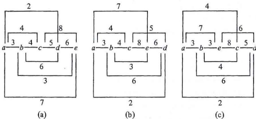
Fig. 10.28. Local optimizations.
