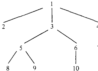
Fig. 3.3. A tree.
