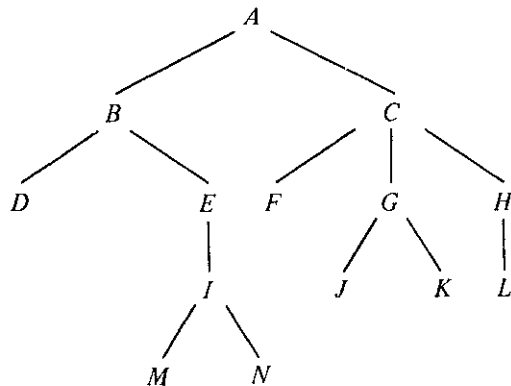
Fig. 3.31. A tree.
