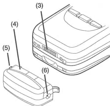
Figure 2-6: Adapter connector
