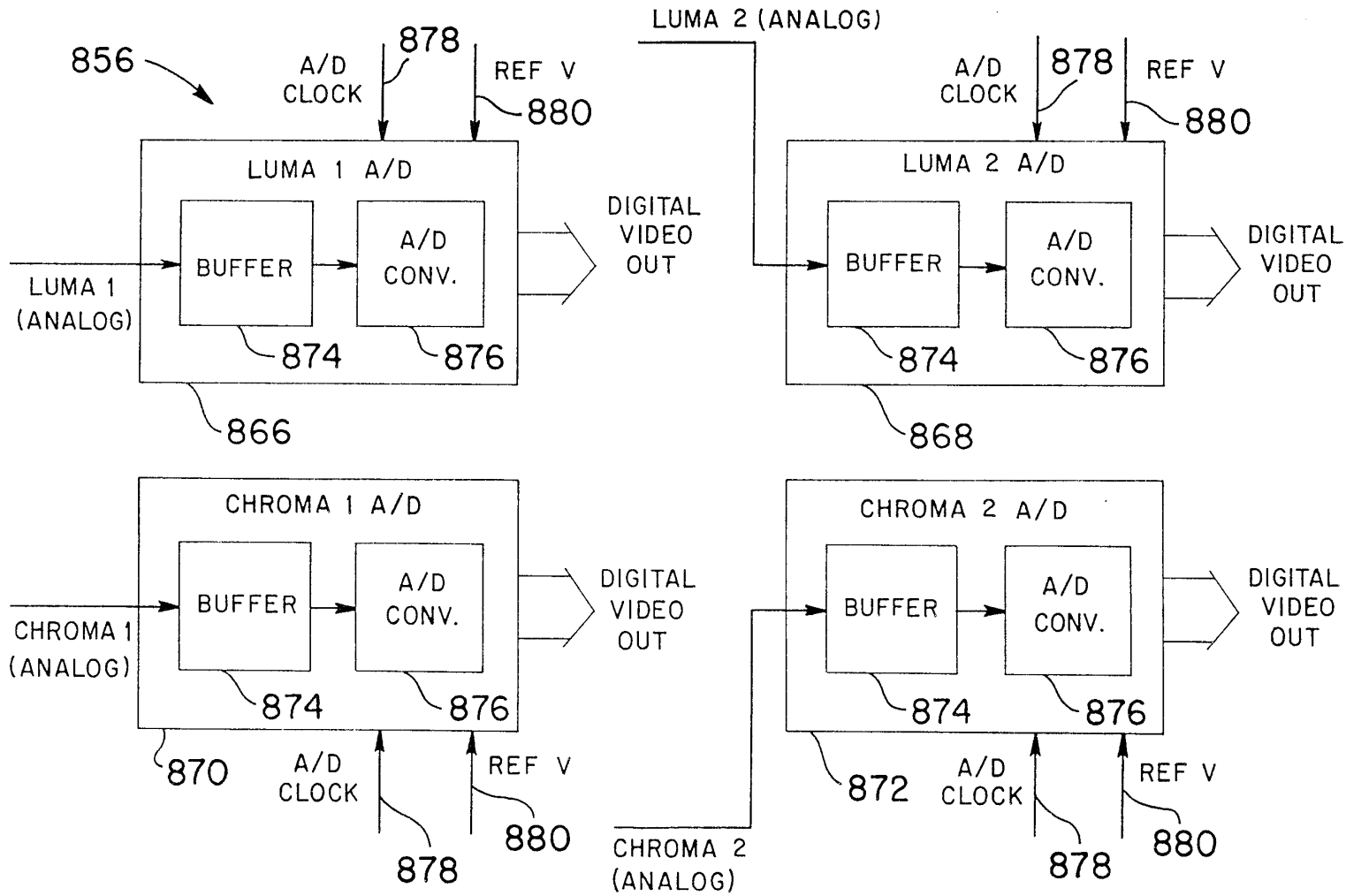
FIG. 16 A/D CONVERSION
