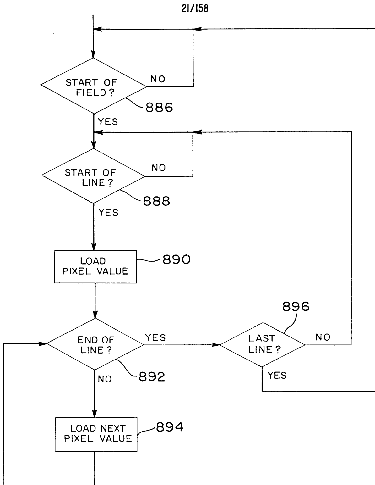
FIG. 17 A CONTROLLER LOGIC (VIDEO DIGITIZING CONTROLLER)
