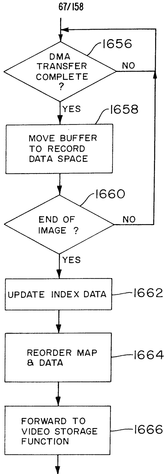
FIG. 71 COMPRESSOR MGR. (VIDEO DATA HANDLING)
