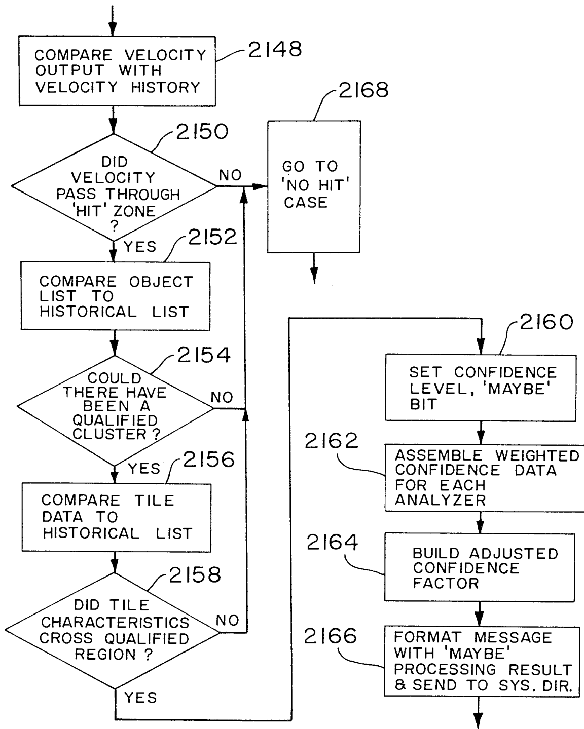
FIG. 95C PROCESSING THE 'MAYBE' CASE
