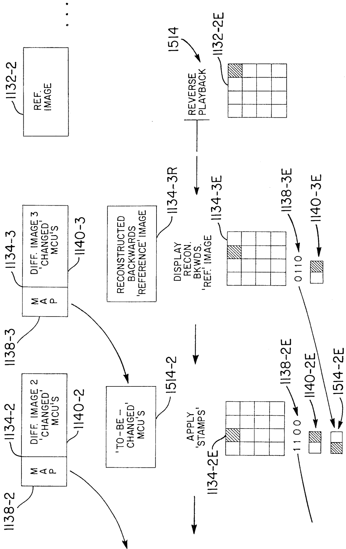
FIG. 64B PICTORIAL ILLUSTRATION OF BACKWARDS DECOMPRESSION
