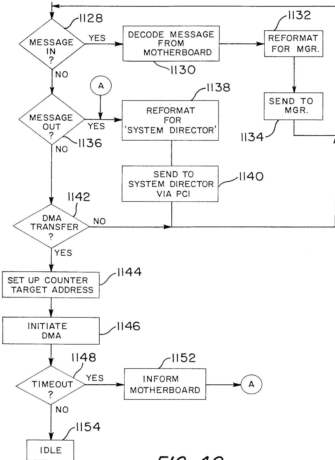
FIG. 40 PCI INTERFACE DRIVER
