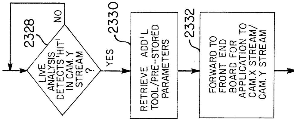
FIG. 106 SOFT-ALARM - ACTUATED LIVE ANALYSIS
