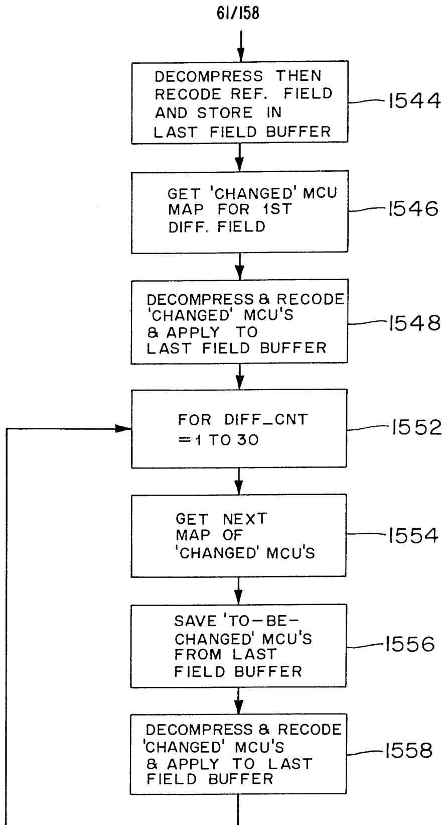
FIG. 66 BUILD BACKWARD HISTORY BUFFER
