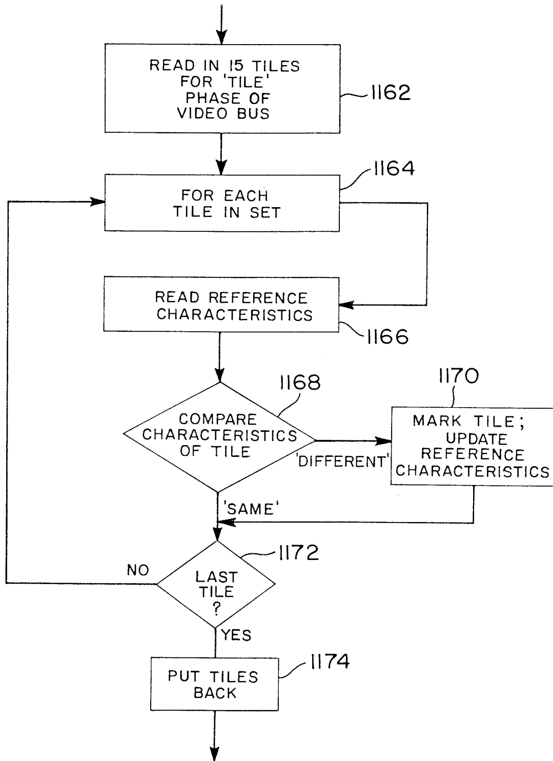
FIG. 42 TILE COMPARING
