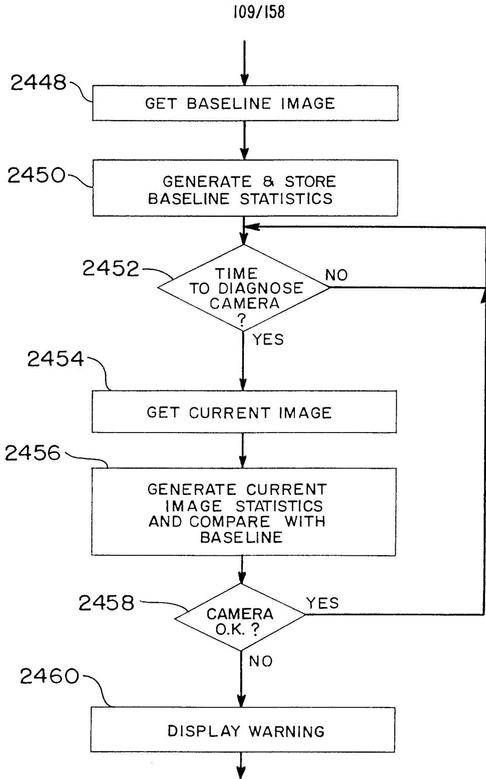
FIG. 120 CAMERA AUTO-DIAGNOSIS
