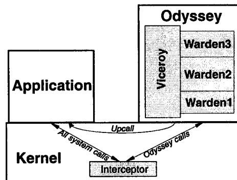
Figure 3. Odyssey architecture
