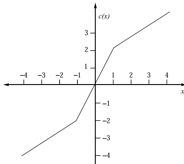
FIGURE 9.23 Compressor mapping.
