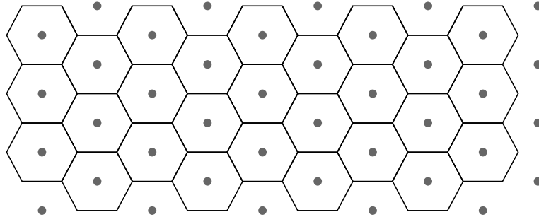
FIGURE 10. 25 The A_2 lattice.
