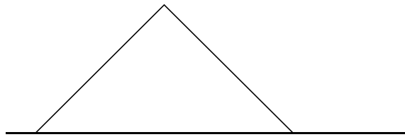
FIGURE 15.9 Triangular scaling function. \blacklozenge
