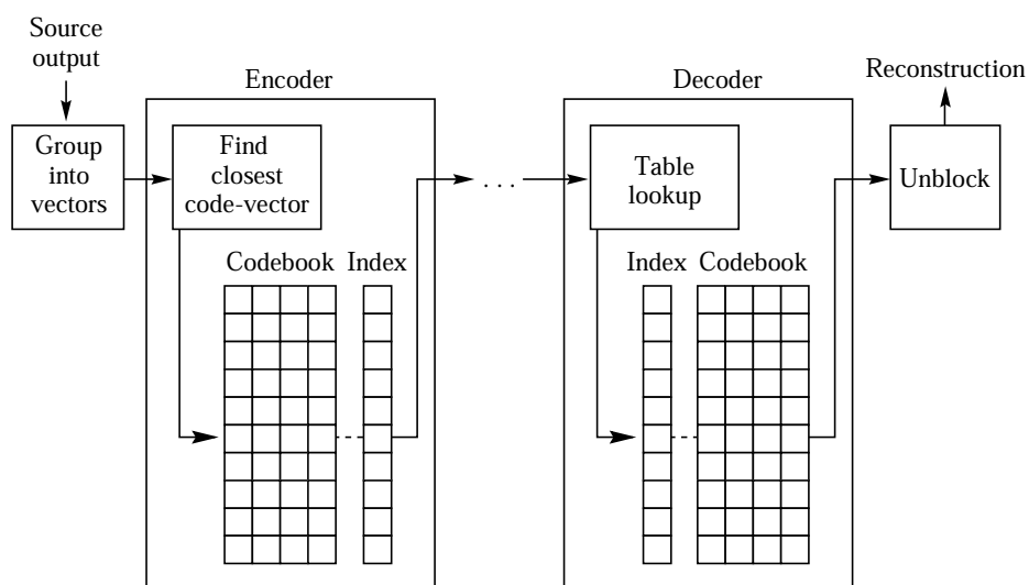
FIGURE 10.1 The vector quantization procedure.
