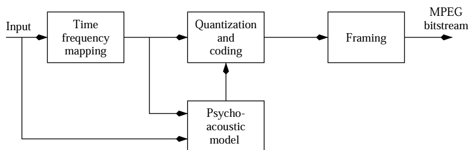
FIGURE 16.4 The MPEG audio coding algorithms.
