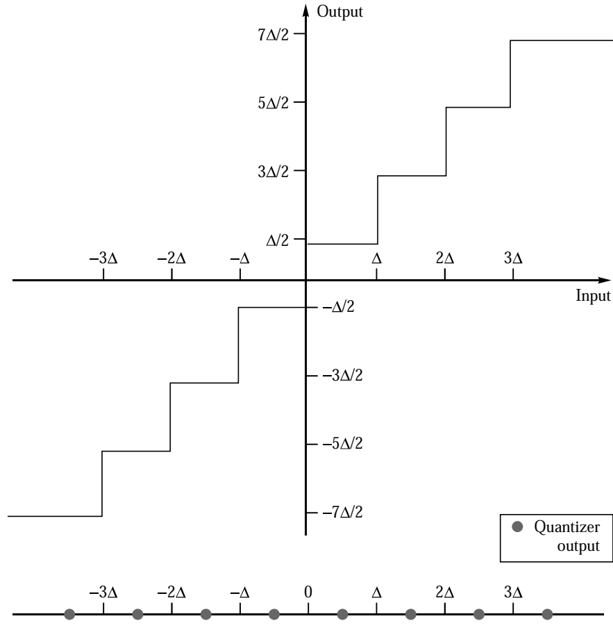
FIGURE 10.4 Two representations of an eight-level scalar quantizer.
