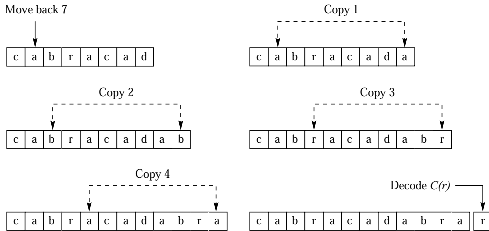
FIGURE 5.3 Decoding the triple \langle 7, 4, C(r) \rangle .
