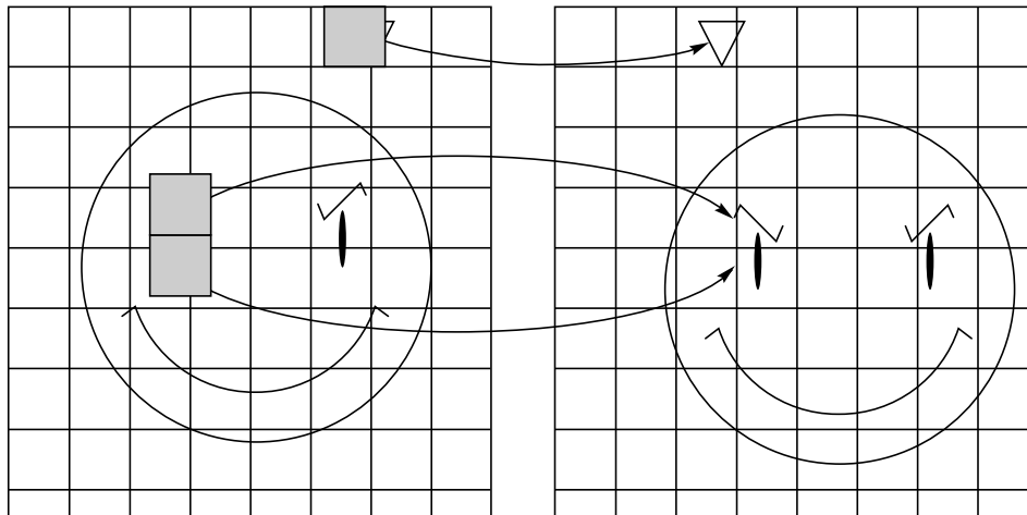
FIGURE 18.3 Motion-compensated prediction.
