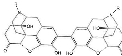
2,2'-Bisnaloxone: R = CH 2 CH=CH 2
