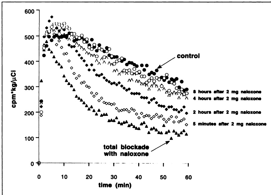
FIGURE 3. Time-activity curves at 5 min ( \blacktriangle ) and 2 ( \blacklozenge ), 4 ( \triangle ) and 8 ( \circ ) hr after the administration of 2 mg of naloxone.
