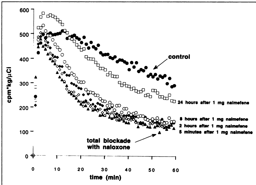
FIGURE 2. Time-activity curves at 5 min ( \diamond ) and 2 ( \Phi ), 8 ( \circ ) and 24 ( \square ) hr after the administration of 1 mg of nalmefene. The radioactivity peaked around 10–15 min after injection of the radiotracer, followed by a slow decline.
