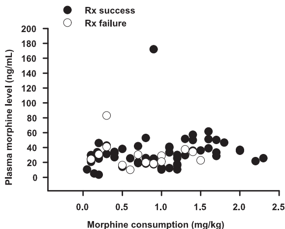
Figure 2. Plasma morphine level as a function of morphine consumption for subjects who achieved adequate symptom control (Rx success, ●) and subjects who failed therapy (Rx failure, ○). At the time the second plasma morphine level was measured, plasma morphine level was independent of morphine consumption for patients in both groups, and average plasma morphine levels did not differ between groups (34.7 \pm 5.1 vs 29.2 \pm 3.2 ng/mL for responders and treatment failures, respectively).
