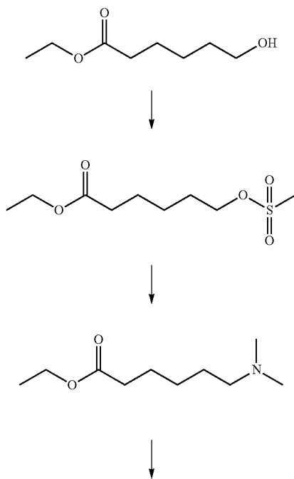
Scheme 14
