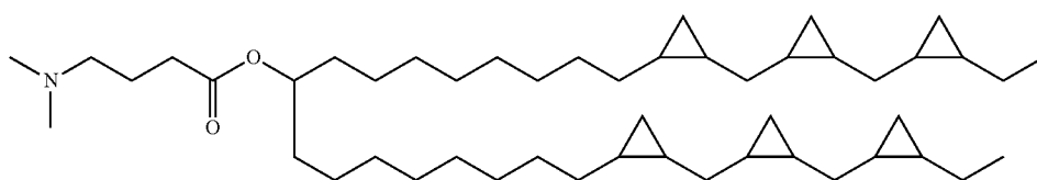
CP-LenMC3
