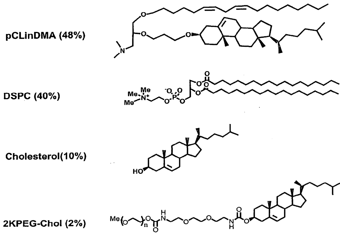
FIGURE 25 Lipid Composition in LNP 083
