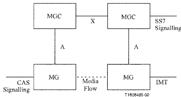
Figure 16/H.323 – Decomposed service provider access and trunking gateways
