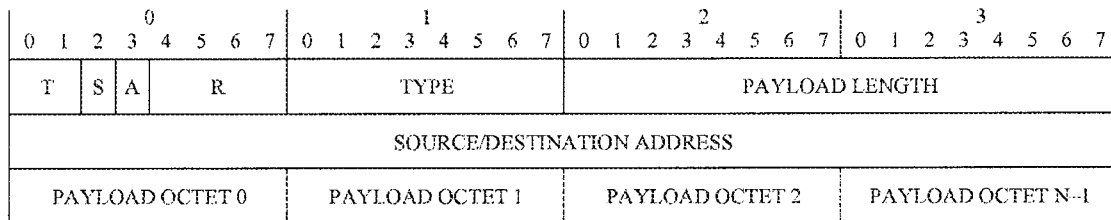
Figure E.17/H.323 – Extended-3 payload format
