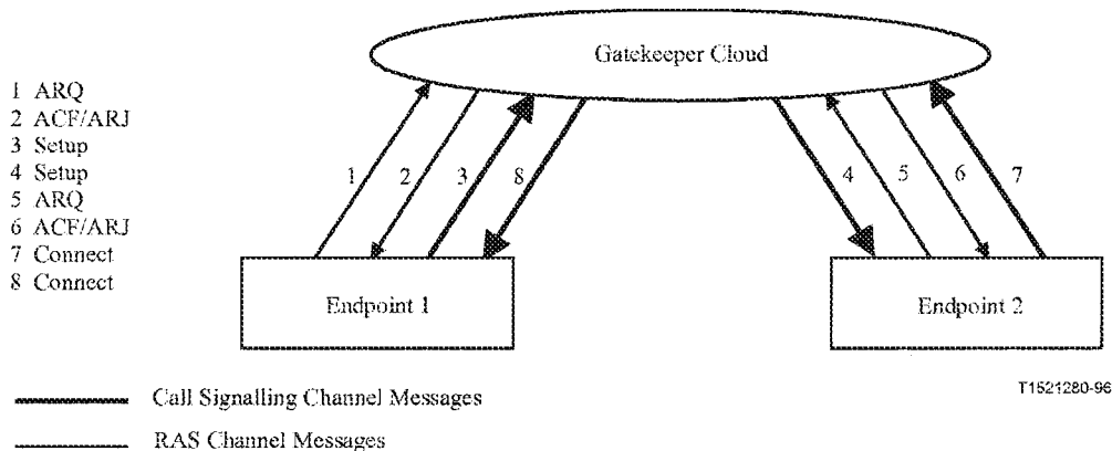
Figure 25/H.323 – Gatekeeper routed call signalling
