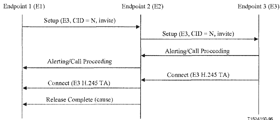
Figure 46/H.323 – Non-MC invite signalling
