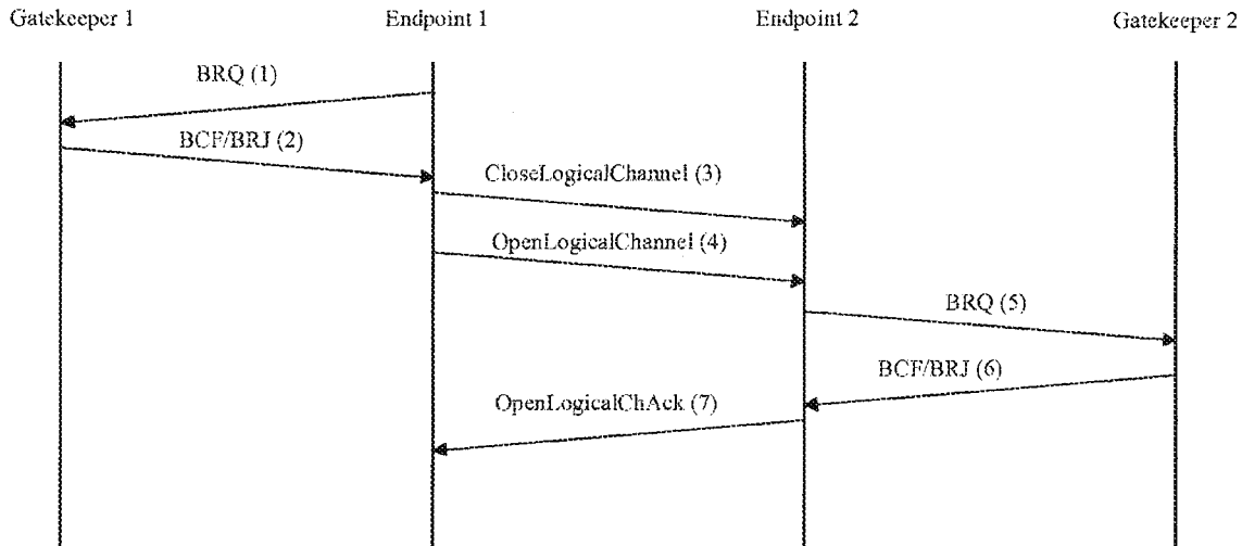
Figure 43/H.323 – Bandwidth change request – Transmitter change
