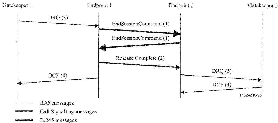
Figure 52/H.323 – Gatekeeper initiated call clearing
