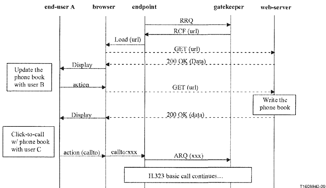
Figure K.4/H.323 – Non-call-related service control
