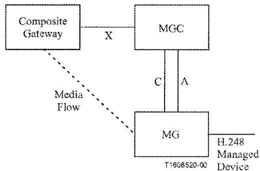
Figure 20/H.323 – Composite gateway and H.248 managed devices
