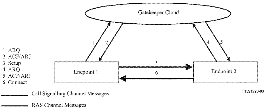
Figure 26/H.323 -- Direct endpoint call signalling
