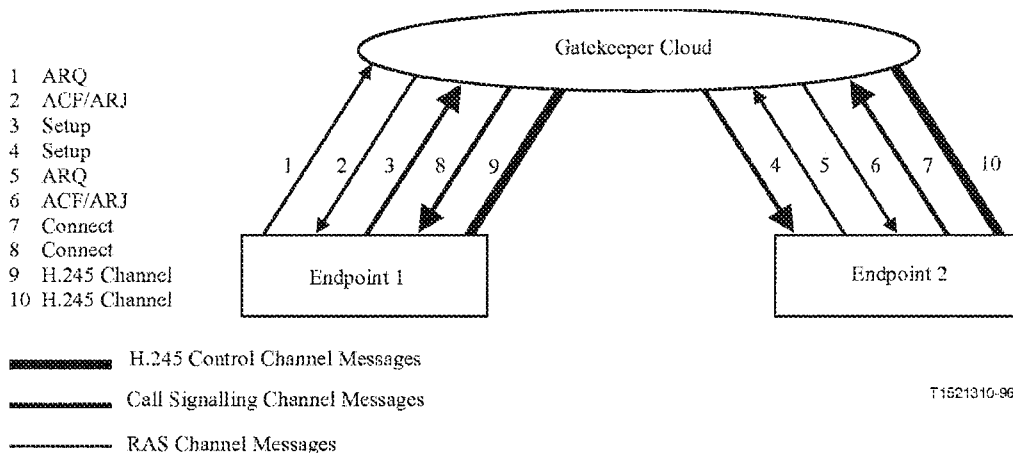
Figure 28/H.323 – Gatekeeper routed H.245 control
