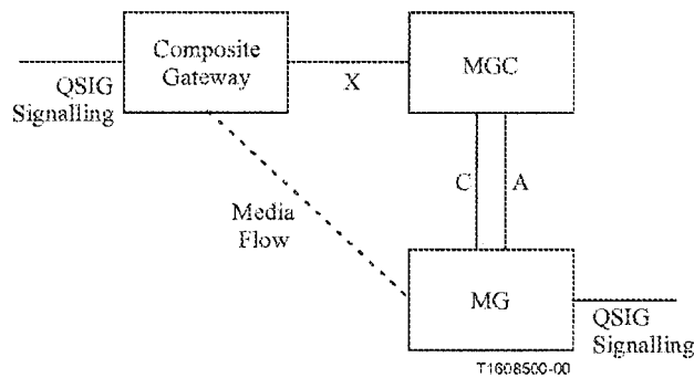
Figure 18/H.323 – QSIG tunnelling example
