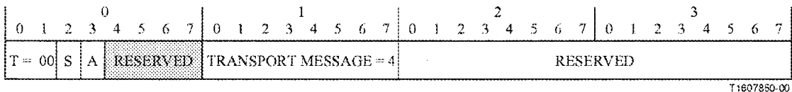
Figure E.12/H.323 – Restart message structure
