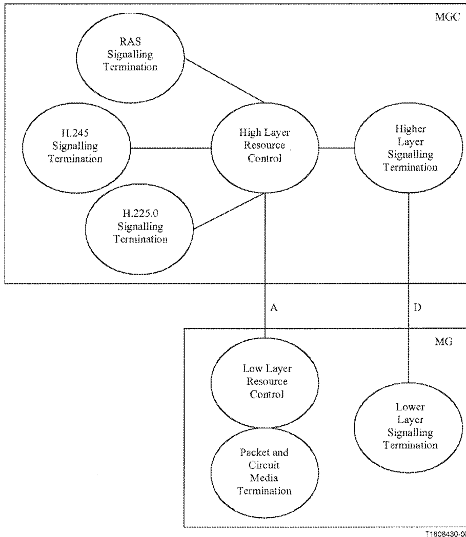
Figure 11/H.323 – SS7 terminated in the MG
