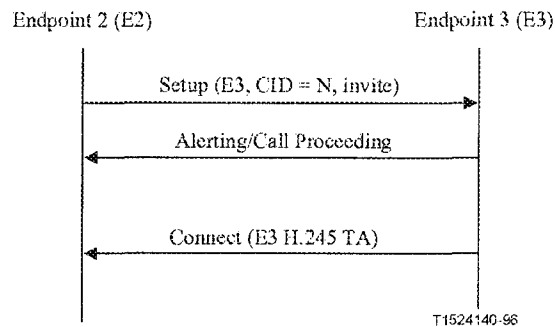
Figure 45/H.323 – MC invite signalling
