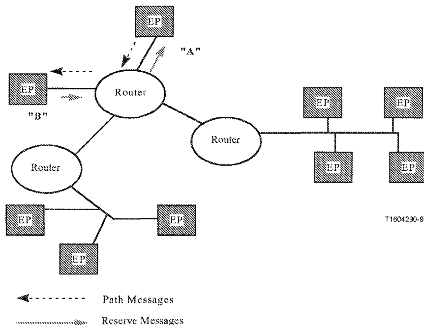
Figure II.1/H.323 – Resource reservation for a point-to-point connection
