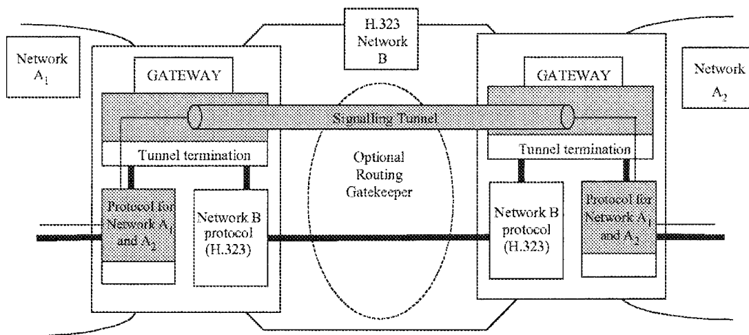
Figure 53/H.323 –Signalling tunnelling between gateways
