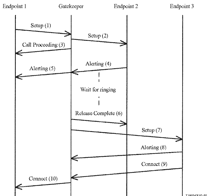
Figure III.1/H.323 – Example of user location using H.225.0/Q.931 signalling (RAS signalling not shown for clarity)
