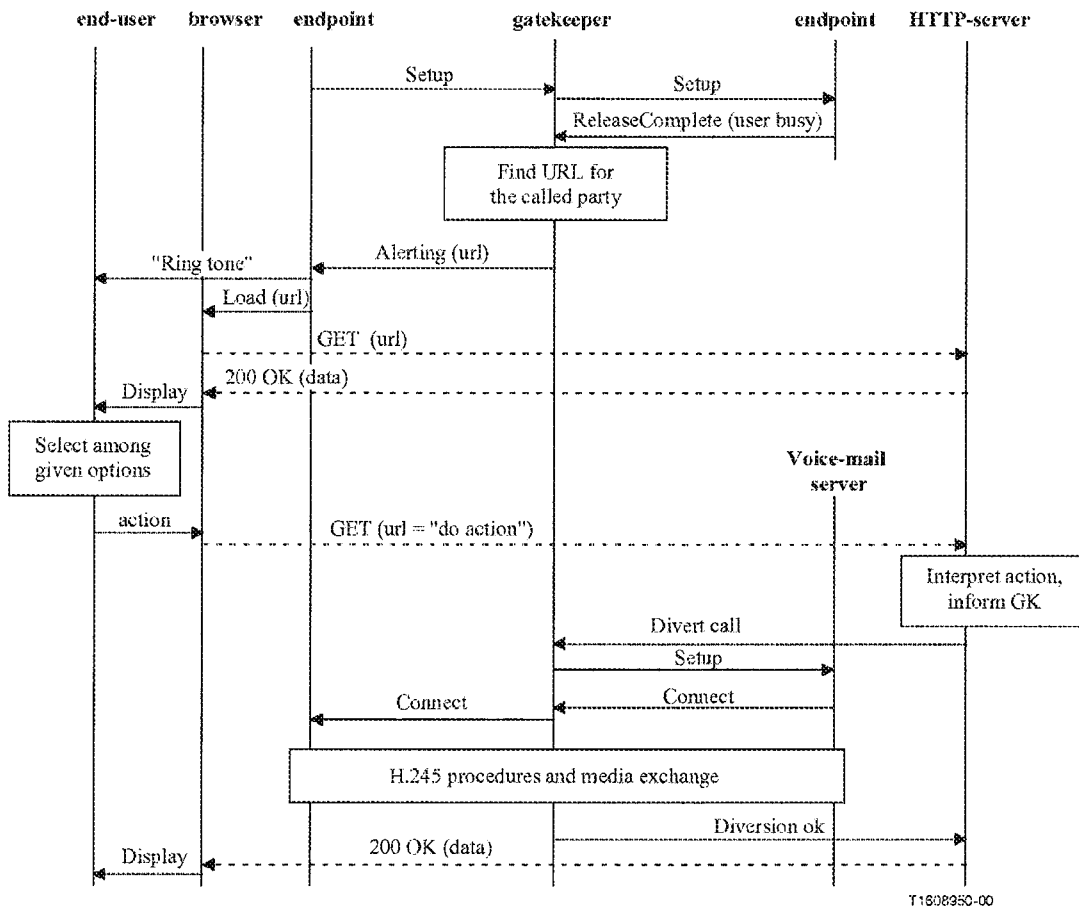
Figure K.5/H.323 – Call-related service control, gatekeeper-routed call
