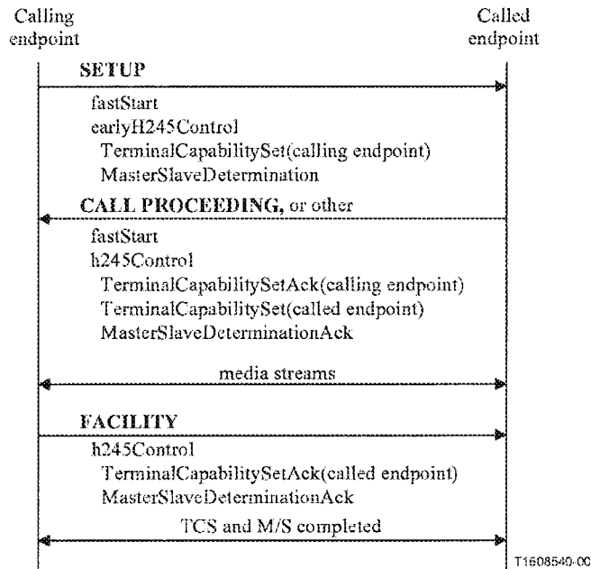
Figure 41/H.323 -- Successful initiation of H.245 in parallel with fast connect
