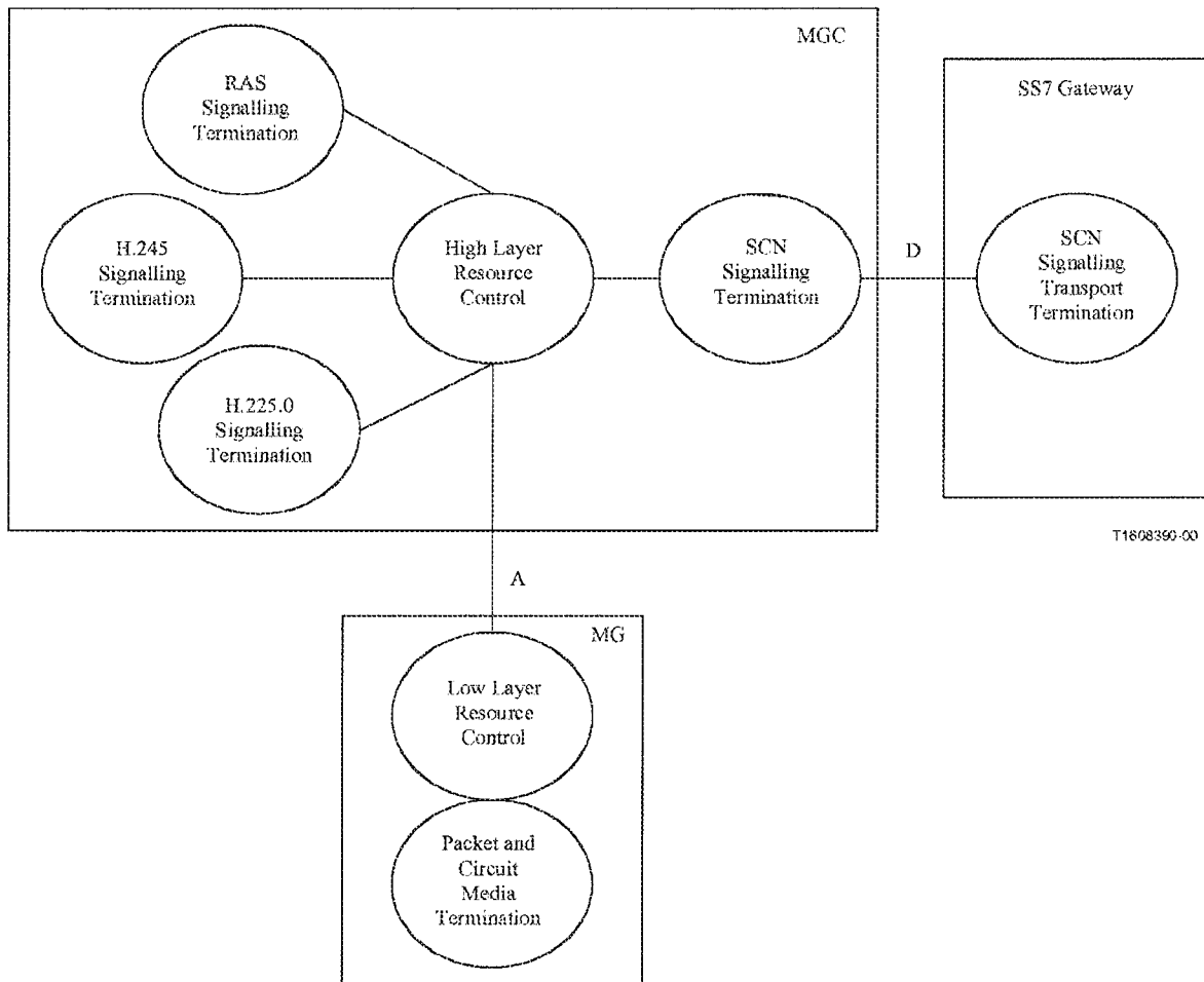
Figure 7/H.323 – SS7 gateway decomposition
