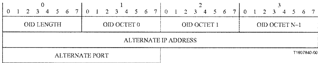
Figure E.11/H.323 – Nack reason 2 structure
