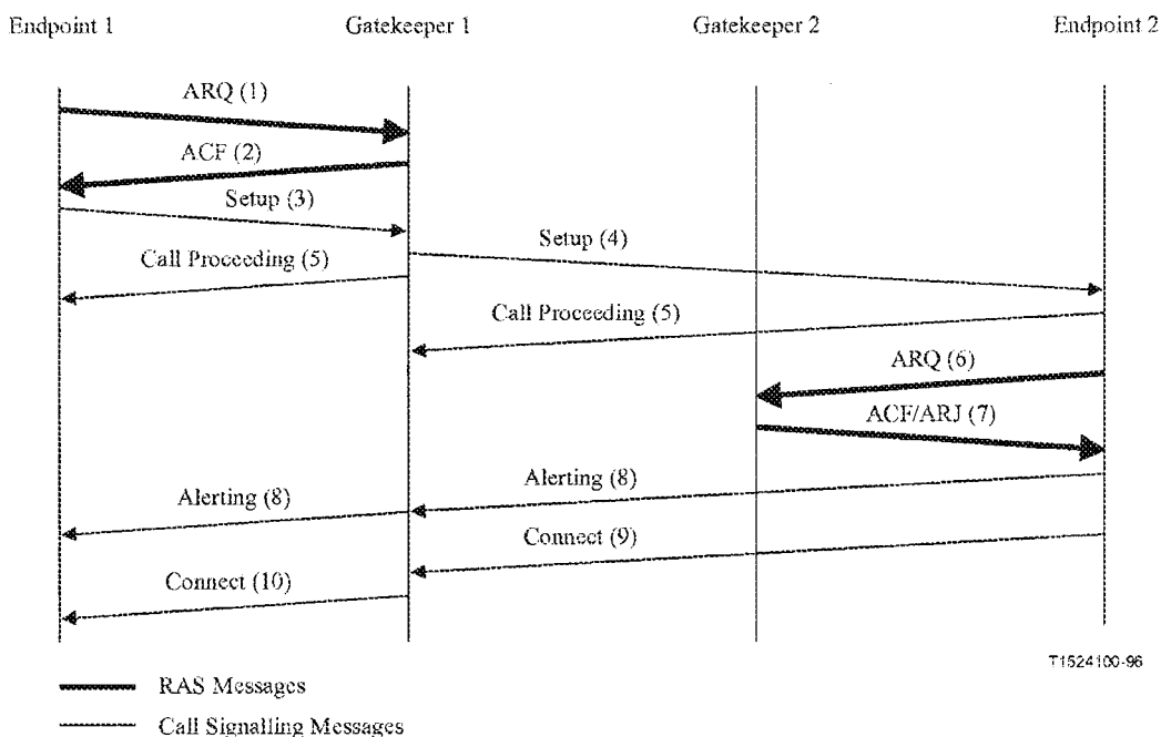
Figure 38/H.323 – Both endpoints registered – Routed/direct call signalling
