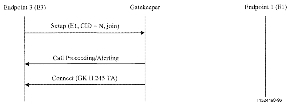
Figure 50/H.323 -- Gatekeeper routed join signalling
