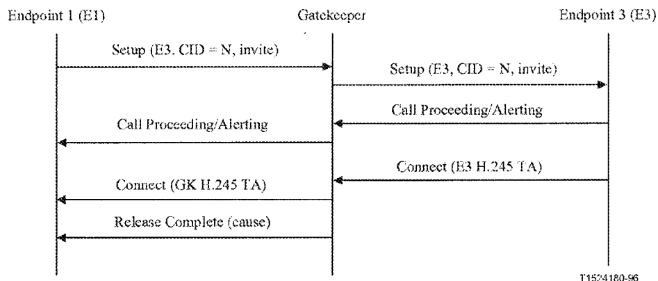
Figure 49/H.323 – Gatekeeper routed invite signalling
