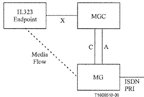
Figure 19/H.323 – Decomposed gateway and H.323 endpoint
