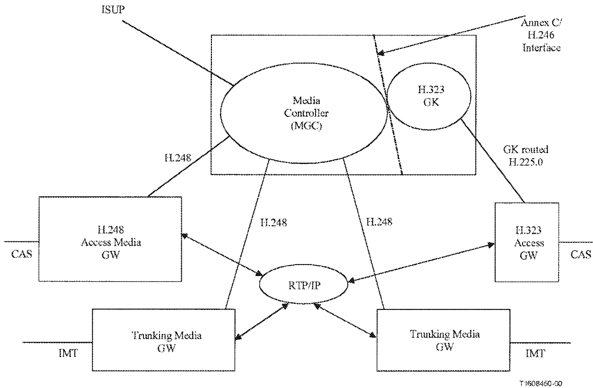
Figure 13/H.323 -- Relationship of H.323 and H.248
