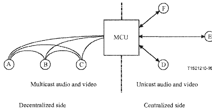
Figure 2/H.323 – Mixed multipoint conference
