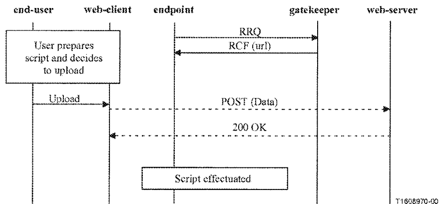
Figure K.7/H.323 – Non-call-related service control, script upload
