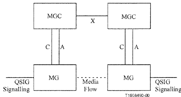
Figure 17/H.323 – Decomposed enterprise trunking gateways
