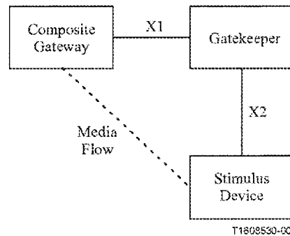
Figure 21/H.323 – Composite gateway and stimulus device
