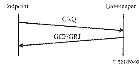
Figure 23/H.323 -- Auto discovery
