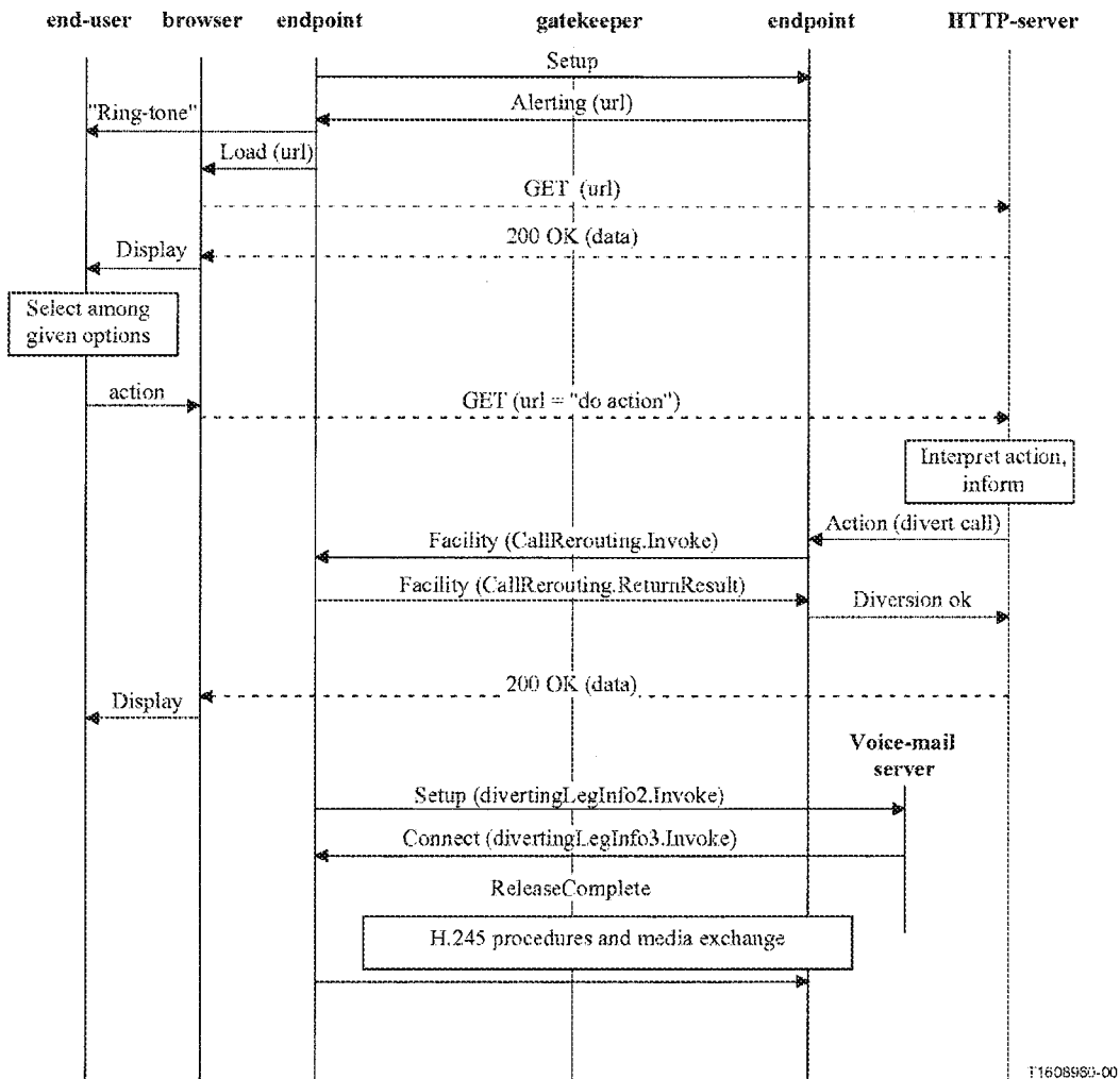
Figure K.6/H.323 – Call-related-service control, non-gatekeeper-routed call
