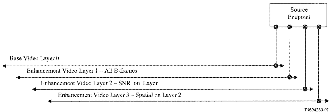
Figure B.1/H.323 – Model with layered video
