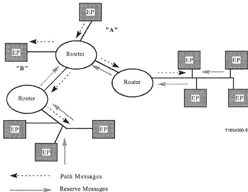
Figure II.2/H.323 -- Resource reservation for a point-to-multipoint connection
