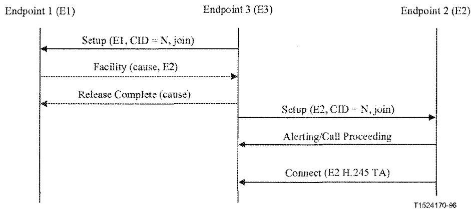
Figure 48/H.323 – Non-MC join signalling
