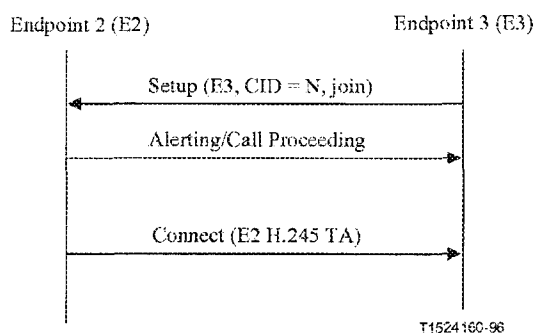
Figure 47/H.323 – MC join signalling
