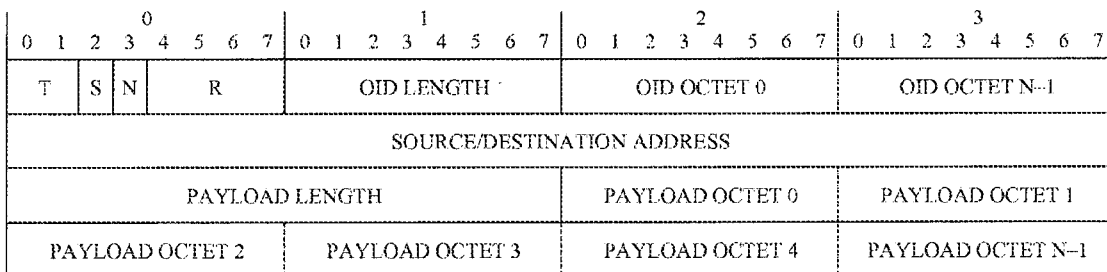
Figure E.21/H.323 – Extended-3 ObjectID-typed payload format
