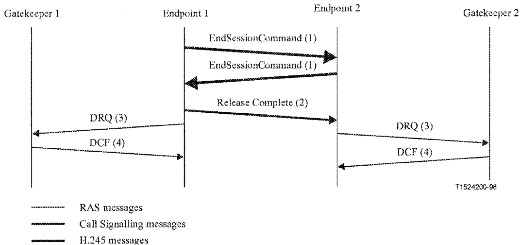
Figure 51/H.323 -- Endpoint initiated call clearing
