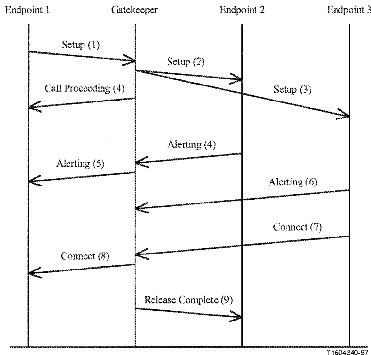
Figure III.2/H.323 – Example of user location using H.225.0/Q.931 signalling (RAS signalling not shown for clarity)
