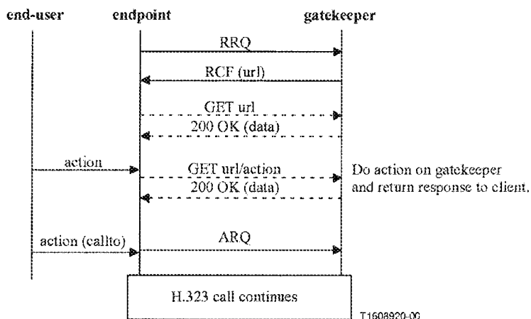
Figure K.2/H.323 – Example of non-call-related service control
