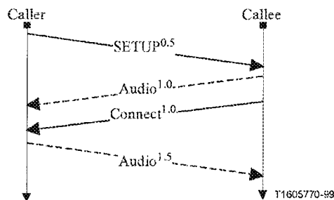
Figure E.23/H.323 – Information flow for UDP-based Call-Setup
