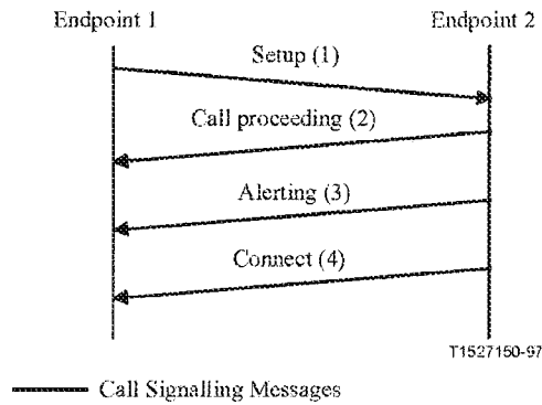
Figure 29/H.323 – Basic call setup, no Gatekeepers
