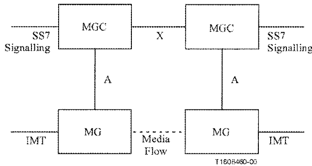
Figure 14/H.323 -- Two decomposed service provider trunking gateways
