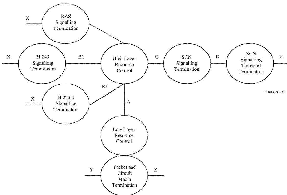
Figure 6/H.323 – Functional architecture of the decomposed gateway
