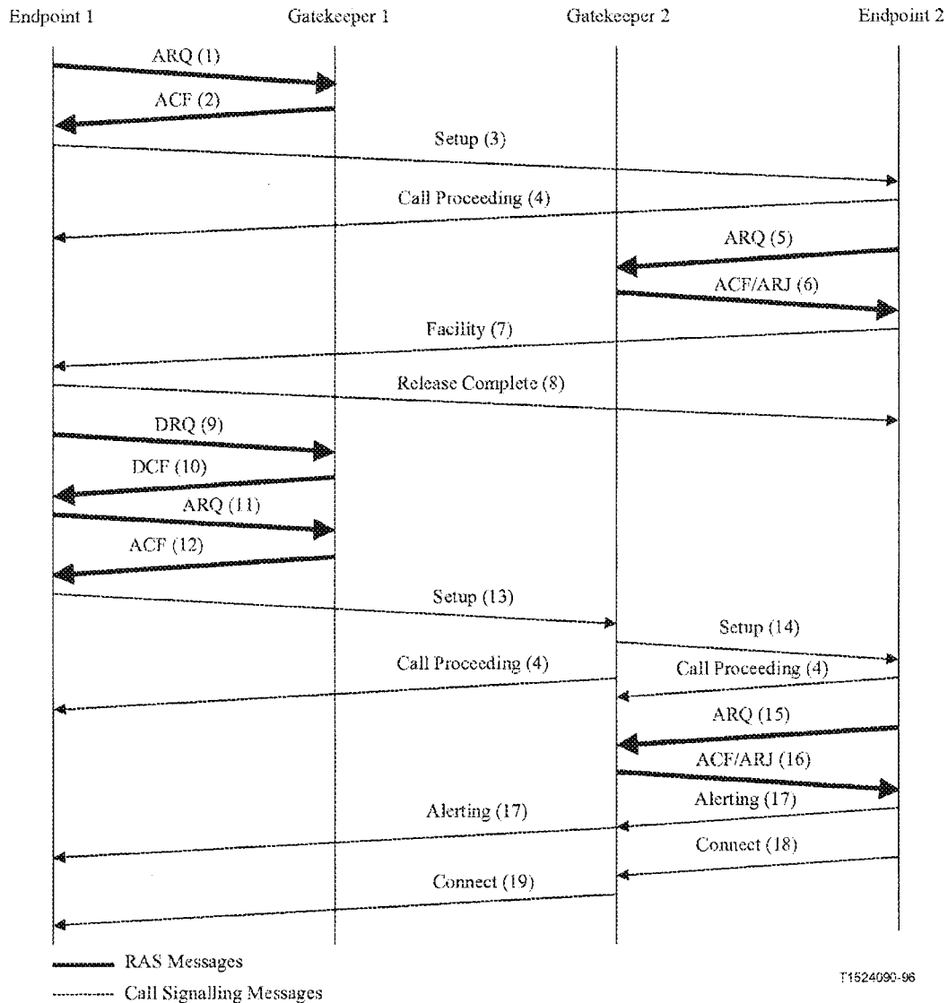
Figure 37/H.323 – Both endpoints registered – Direct/routed call signalling
