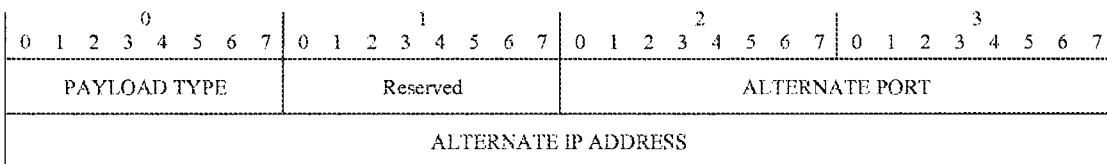
Figure E.10/H.323 – Nack reason 1 structure
