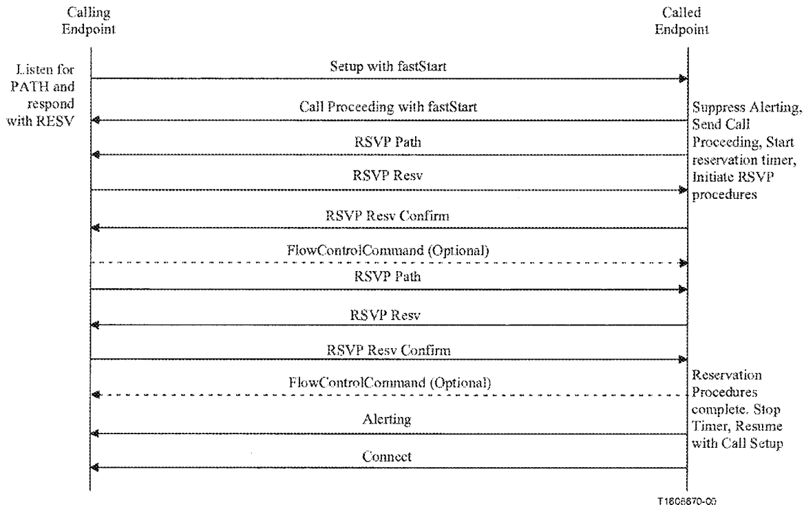
Figure II.6/H.323 -- Synchronizing RSVP when using Fast Connect
