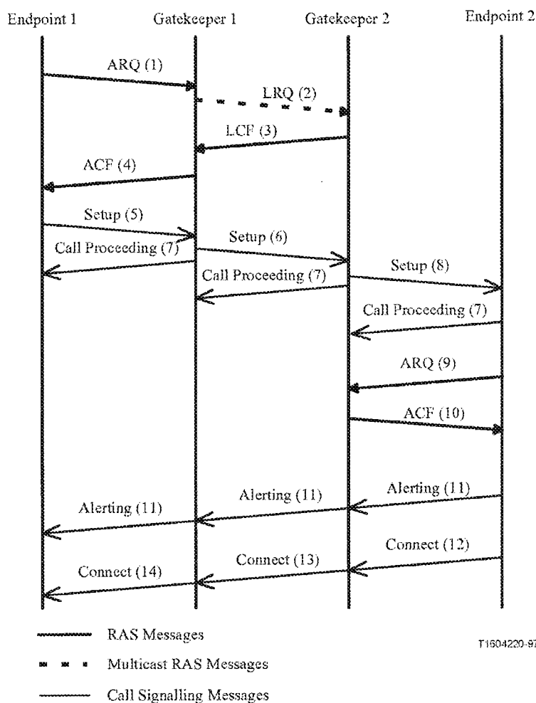
Figure 40/H.323 -- Optional called endpoint signalling
