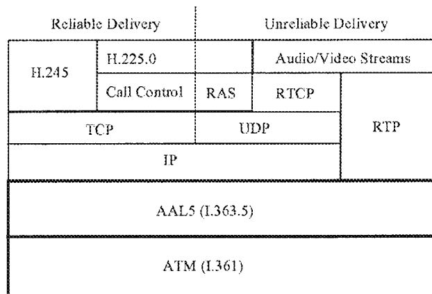
Figure C.1/H.323 – Architecture for H.323 on ATM-AAL5
