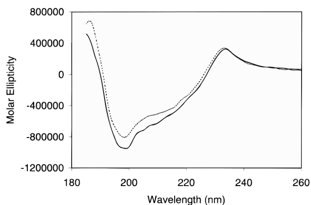
Fig. 4. Far-UV CD spectra of oxidized (---) and control (—) BDNF. (Molar ellipticity: [\Theta] , dec cm 2 dmol -1 ).
