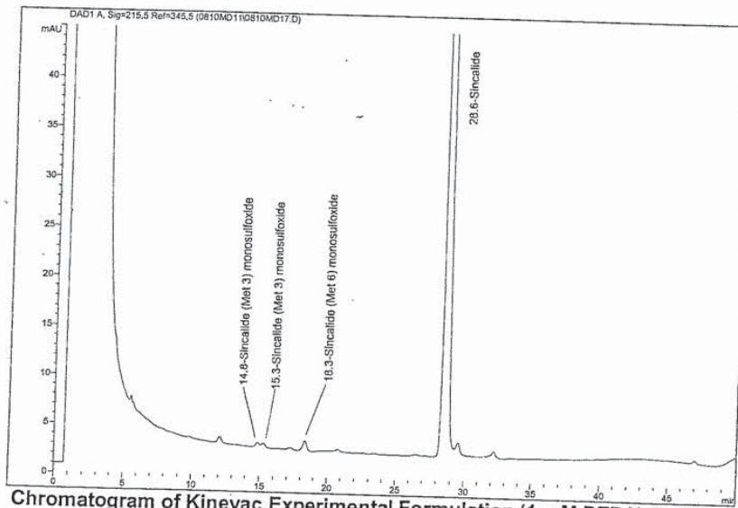
Chromatogram of Kinevac Experimental Formulation (1 mM DTPA) Spiked with 0.63 mM Cu 2+
