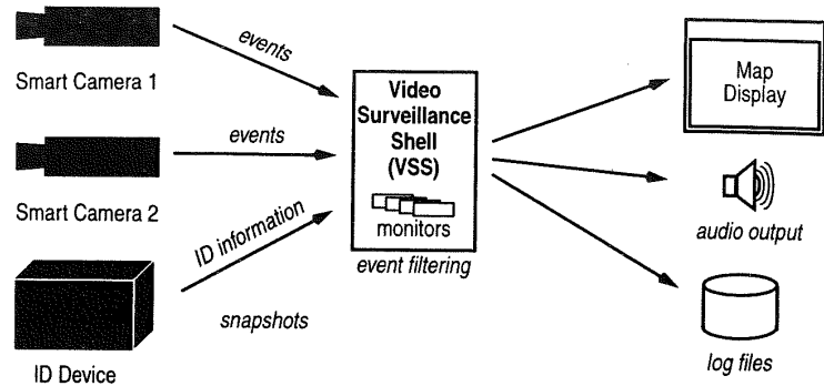
Figure 1: AVS system diagram
