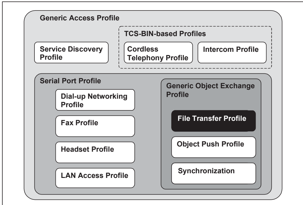
Figure 1.1: Bluetooth Profiles
