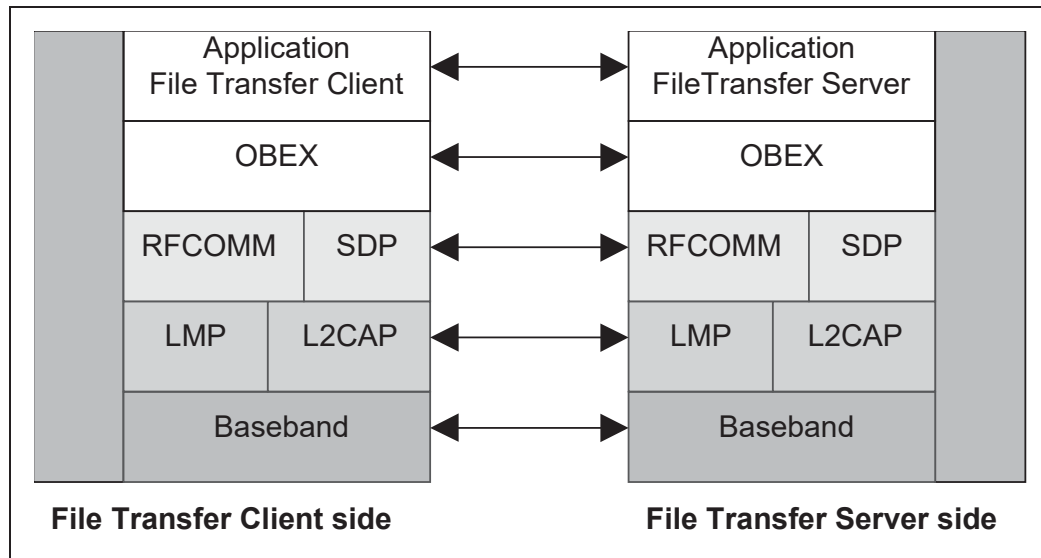
Figure 2.1: Protocol model
