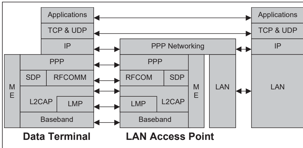
Figure 2.1: Protocol Stack
