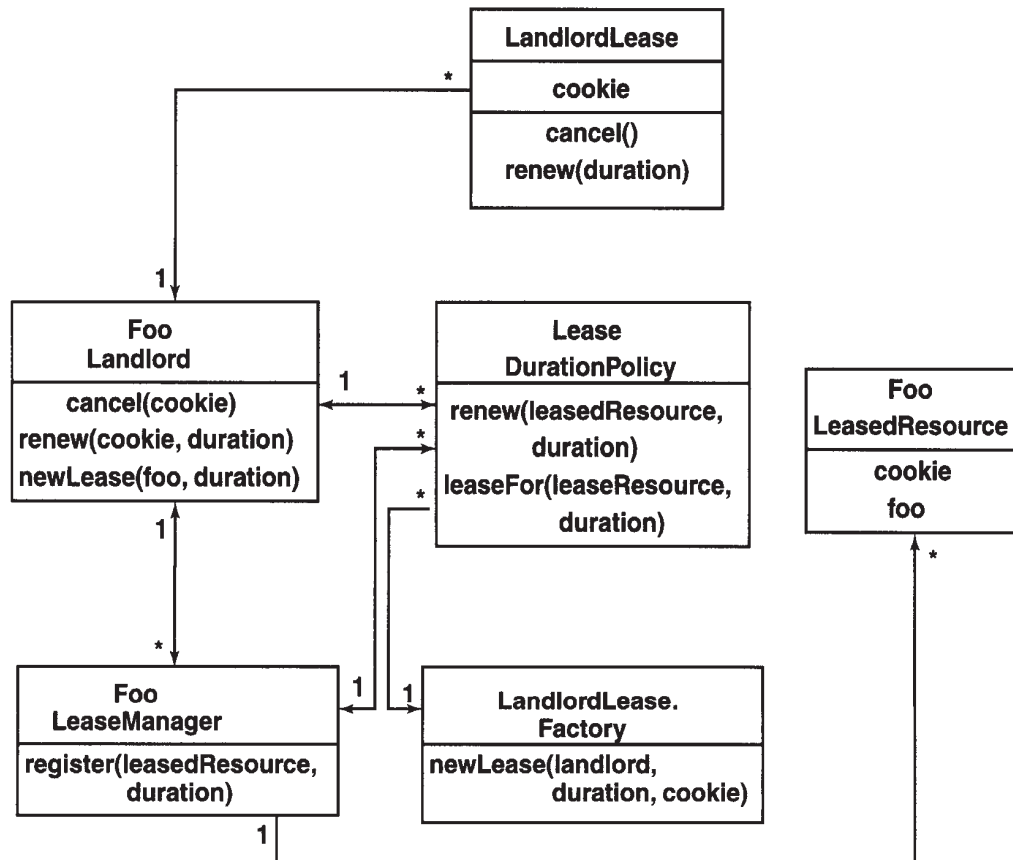
Figure 7-3. Class diagram of a landlord implementation
