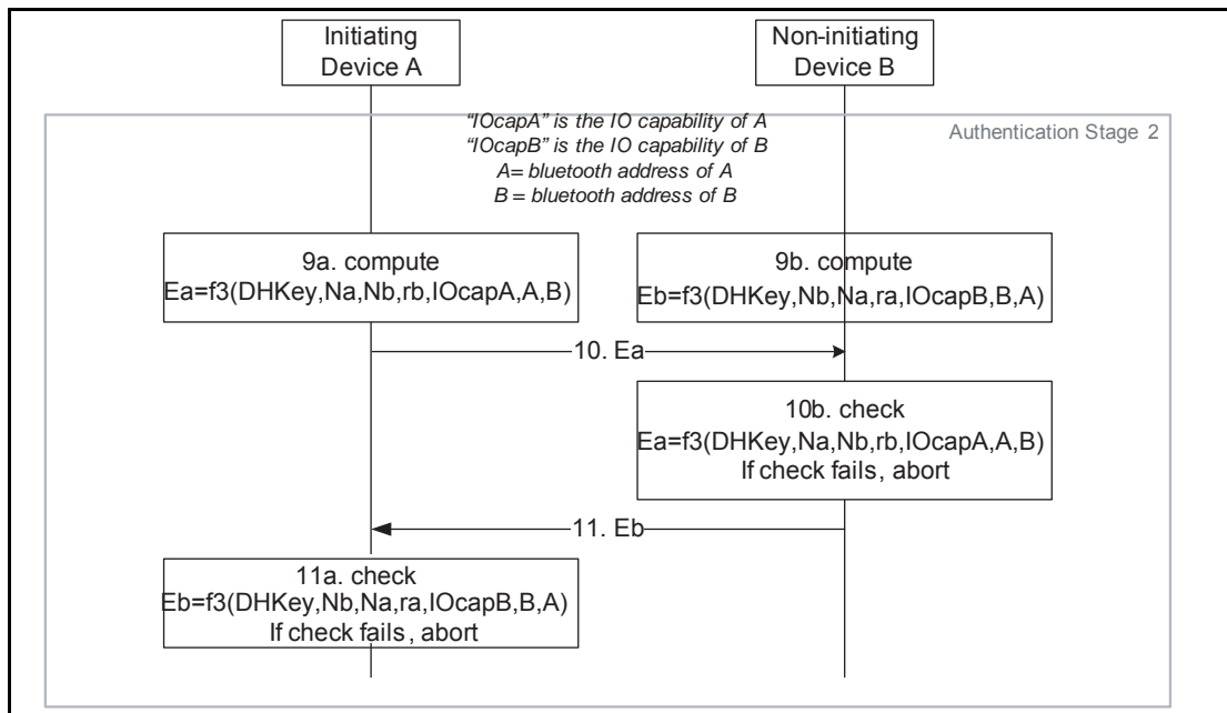
Figure 7.7: Authentication Stage 2
