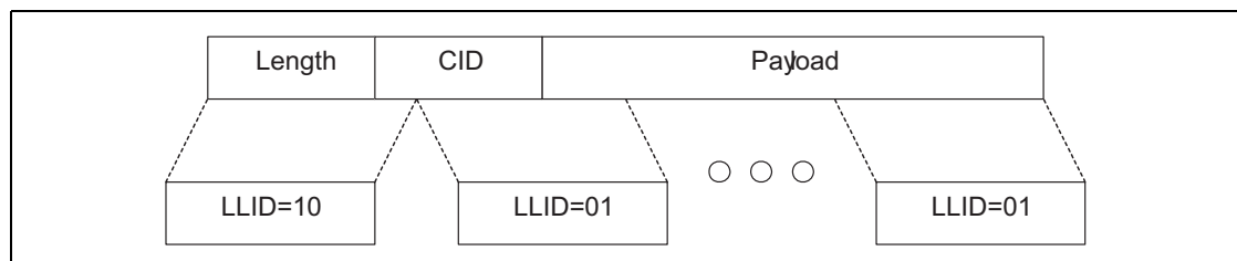
Figure 7.1: L2CAP fragmentation.
