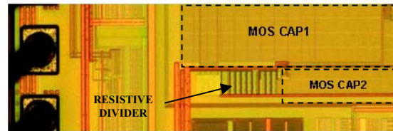
Figure 4. Die photograph of the proposed RF attenuator.
