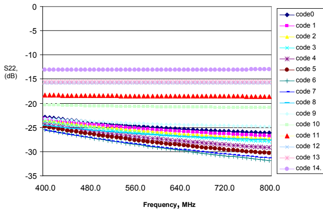
Figure 5. Measured output matching ( S_{22} ) for different gain code settings. The frequency was swept from 400 MHz to 800 MHz.
