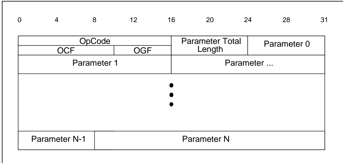
Figure 4.1: HCI Command Packet
