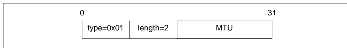
Figure 6.2: MTU Option Format
