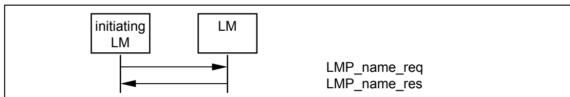
Sequence 70: Device's name requested and it responds.
