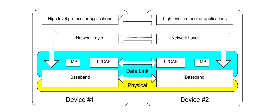
Figure 1.1: L2CAP within protocol layers
