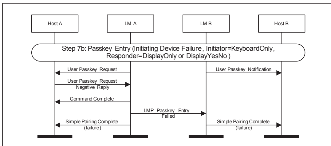
Figure 4.15: Passkey Entry Failure on Initiating Side
