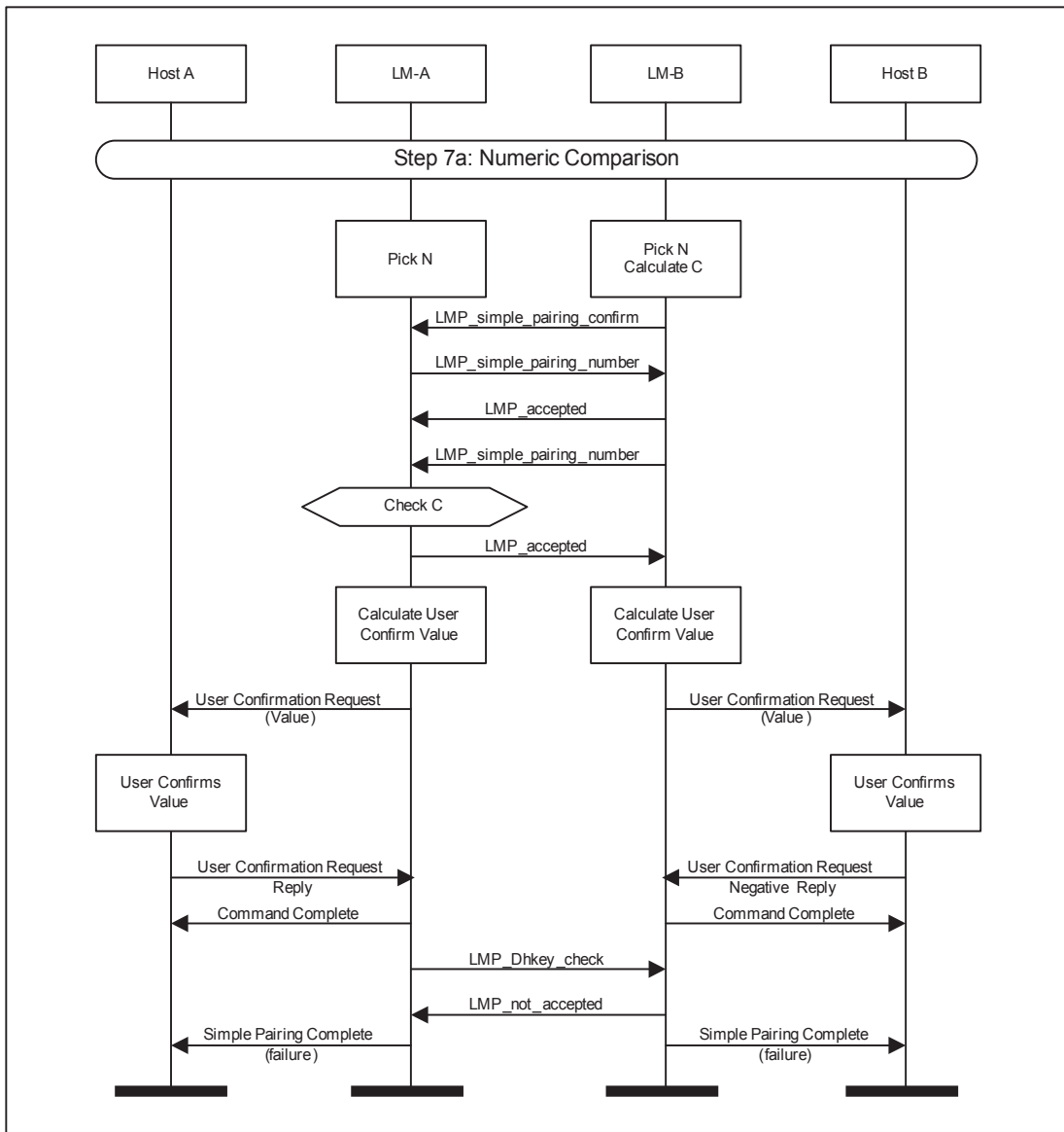
Figure 4.12: Numeric Comparison Failure on Responding Side
