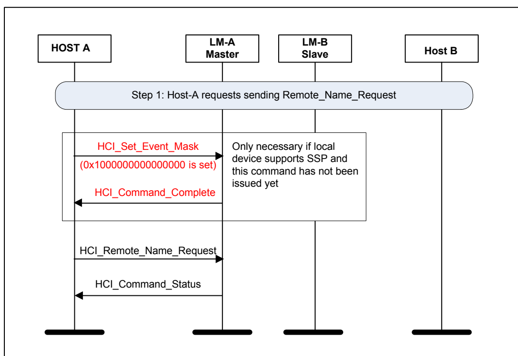
Figure 2.1: Remote name request.
