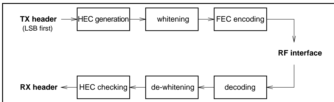
Figure 7.1: Header bit processes.
