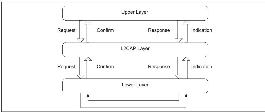
Figure 2.2: L2CAP transaction model.
