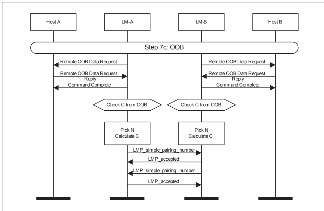
Figure 4.16: OOB Authentication
