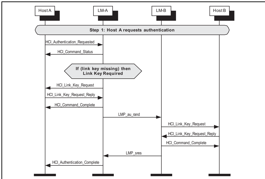
Figure 4.1: Authentication requested.
