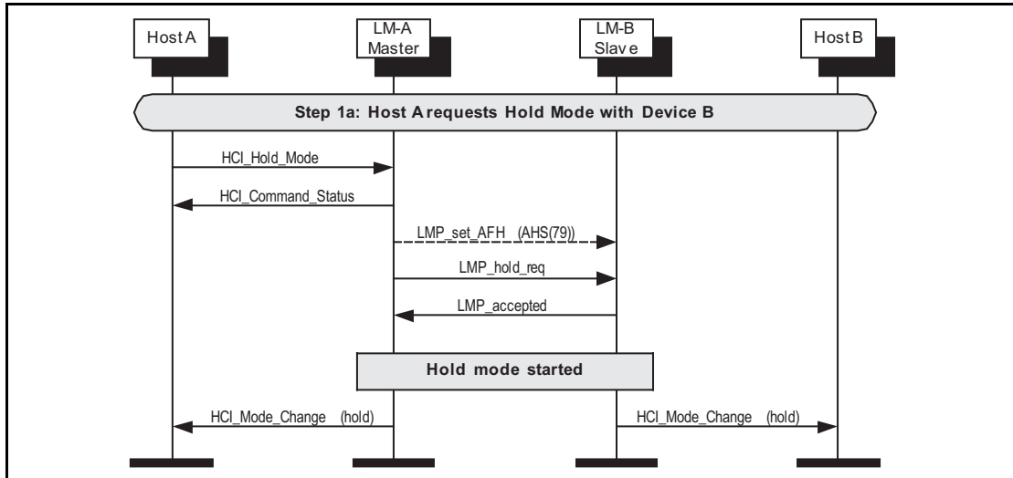
Figure 6.3: Hold request.
