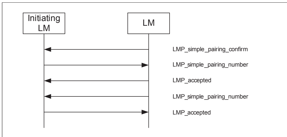
Sequence 47: Numeric Comparison Authentication: Commitment check success
