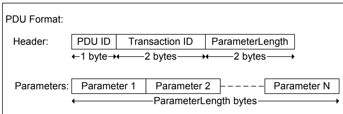
Figure 4.1:
