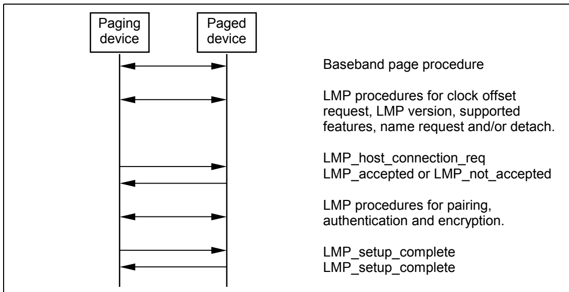
Figure 4.1: Connection establishment.
