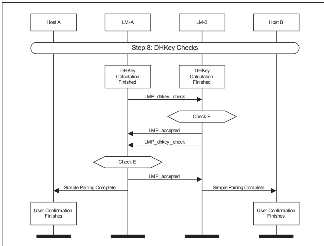
Figure 4.18: DHKey Checks
