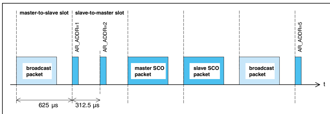
Figure 8.17: Disturbance of access window by SCO traffic
