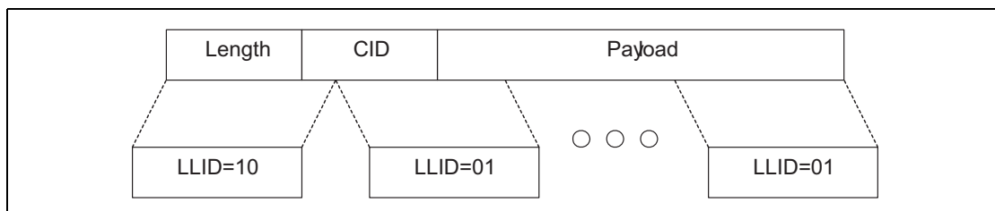
Figure 7.1: L2CAP fragmentation.
