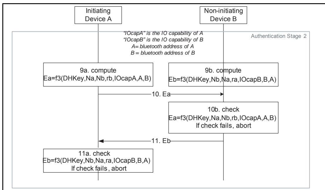
Figure 7.7: Authentication Stage 2
