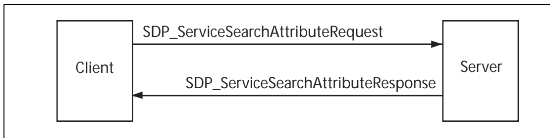
Figure 4.6:
