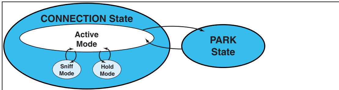
Figure 8.5: Connection state.
