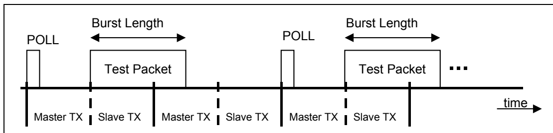
Figure 1.2: Timing for Transmitter Test
