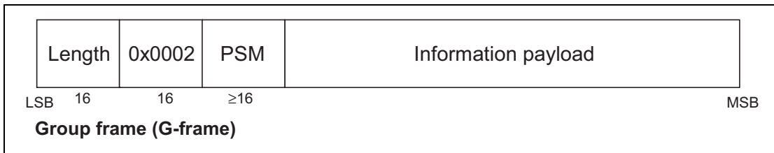
Figure 3.2: L2CAP PDU format in Basic L2CAP mode on Connectionless channel
