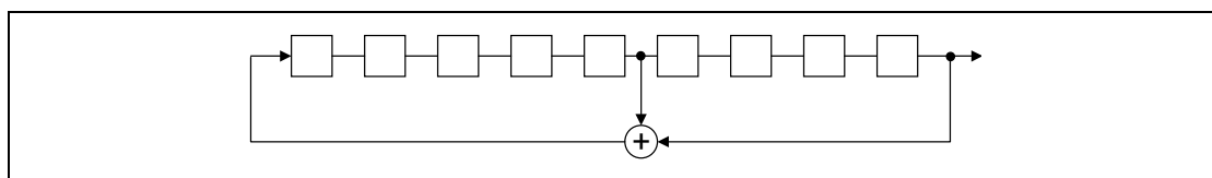
Figure 1.5: Linear Feedback Shift Register for Generation of the PRBS sequence
