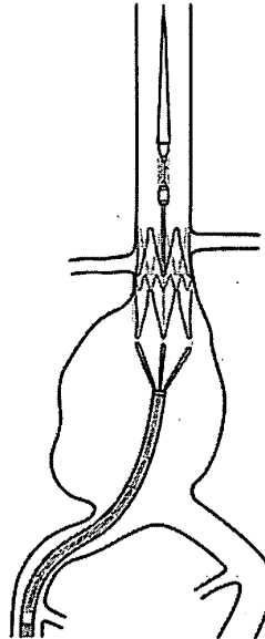
Figure 10: Deploy the Proximal End
