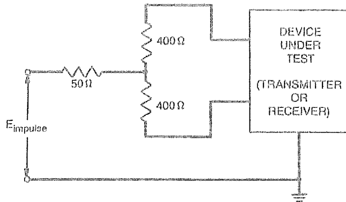
Fig 12-27 Common-Mode Impulse Test
