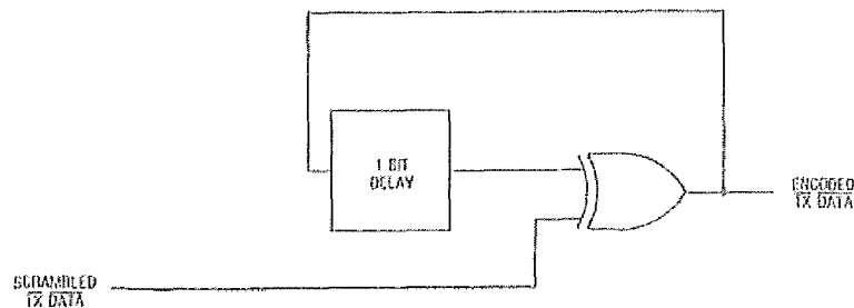
Fig 11-11 Differential Encoder
