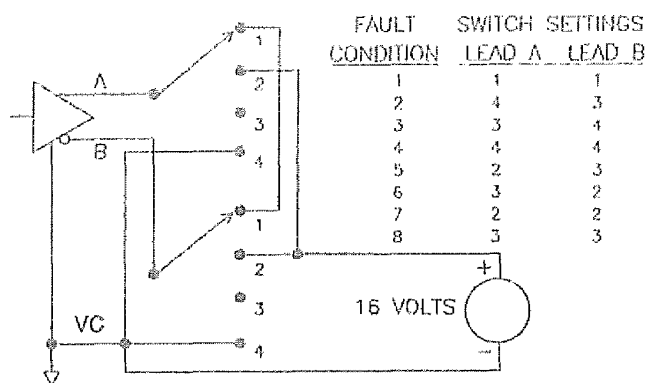
Fig 7-14 Driver Fault Conditions
