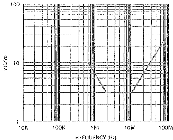
Fig 7-17 Common-Mode Transfer Impedance
