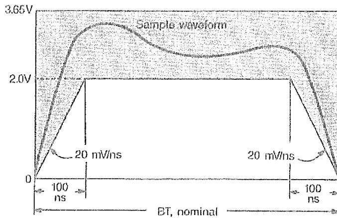
Fig 12-20 Differential Output Voltage, Duration BT
