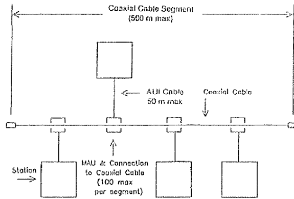
Fig 8-11 Minimal System Configuration
