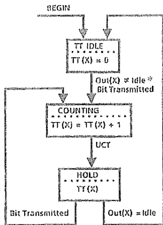
Fig 9-3 Transmit Timer State Diagram for Port X
