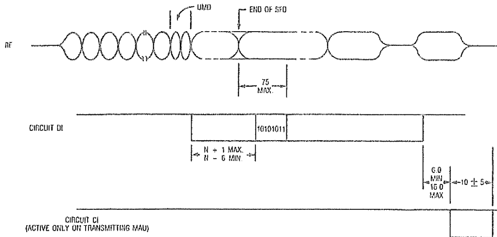
Fig 11-13 No Collision Timing Diagram (Coax to AUI)
