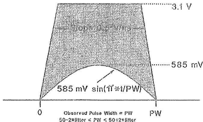
Fig 14-16 Receiver Differential Input Voltage—Narrow Pulse
