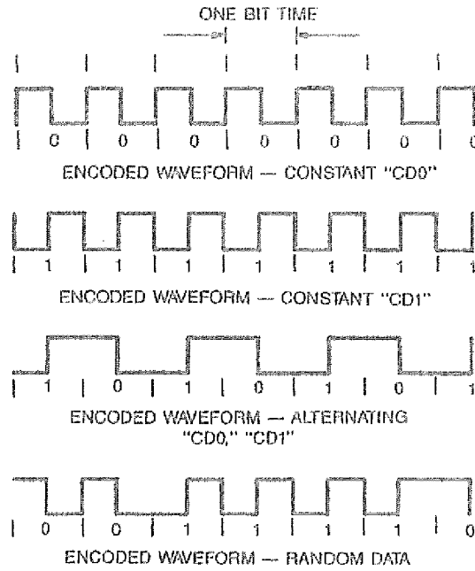
Fig 12-10 Examples of Manchester Waveforms
