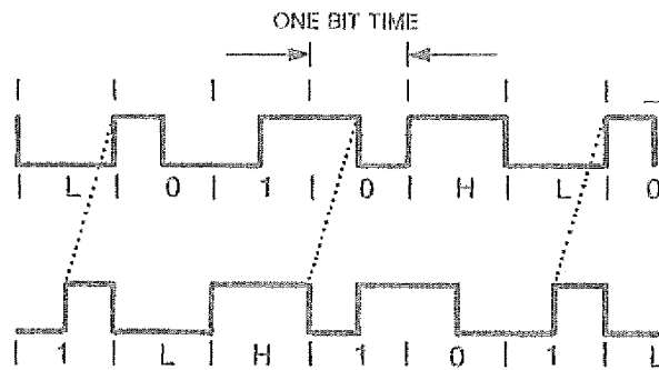
Fig 12-11 Examples of Collision Presence Waveforms
