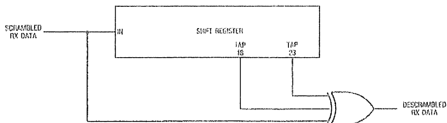
Fig 11-12 Descrambler
