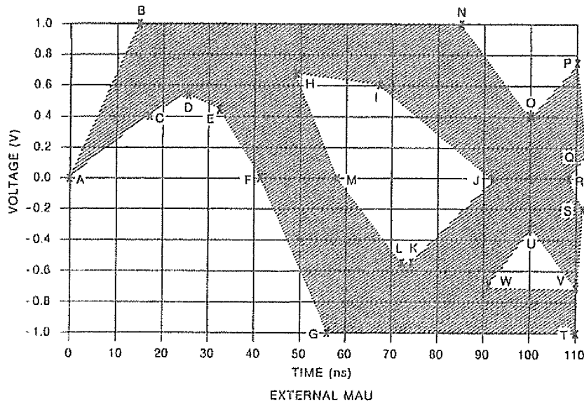
Fig 14-9 Voltage Template
