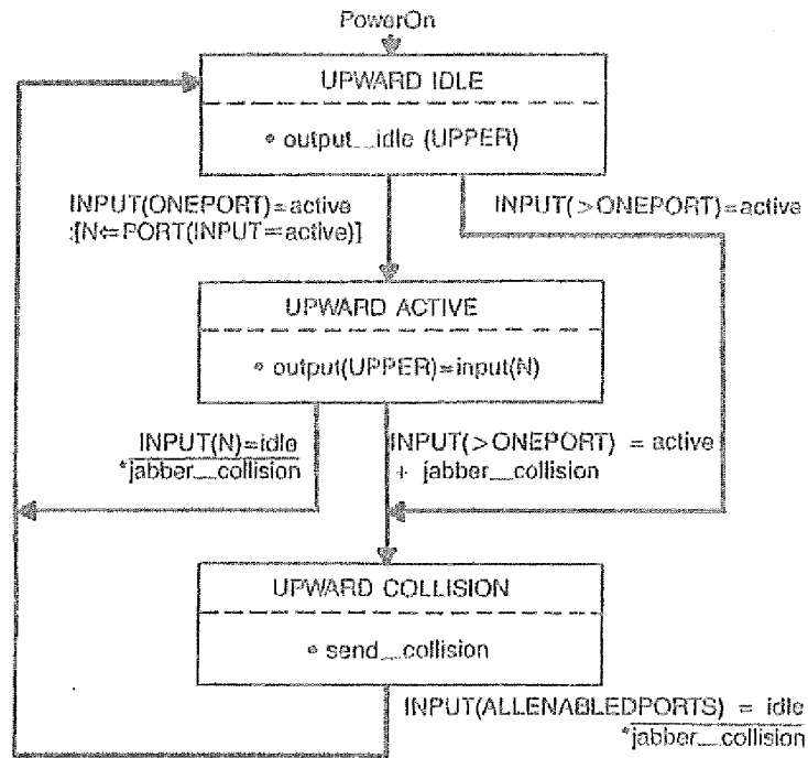
Fig 12-13 Hub PLS Upward Transfer Function
