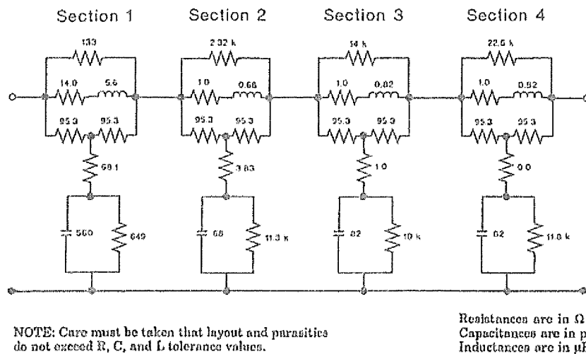
Fig 14-7 Twisted-Pair Model
