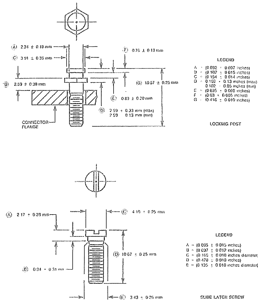
Fig 7-18 Connector Locking Posts
