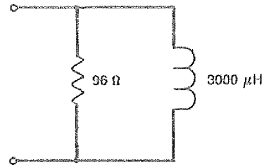
Fig 12-23 Start-of-Idle Test Load #2
