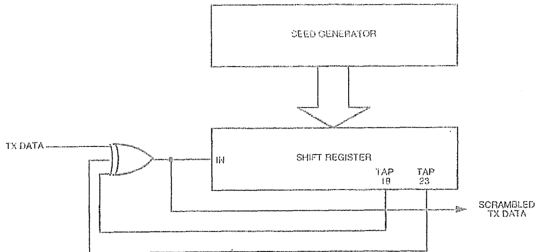
Fig 11-10 Scrambler
