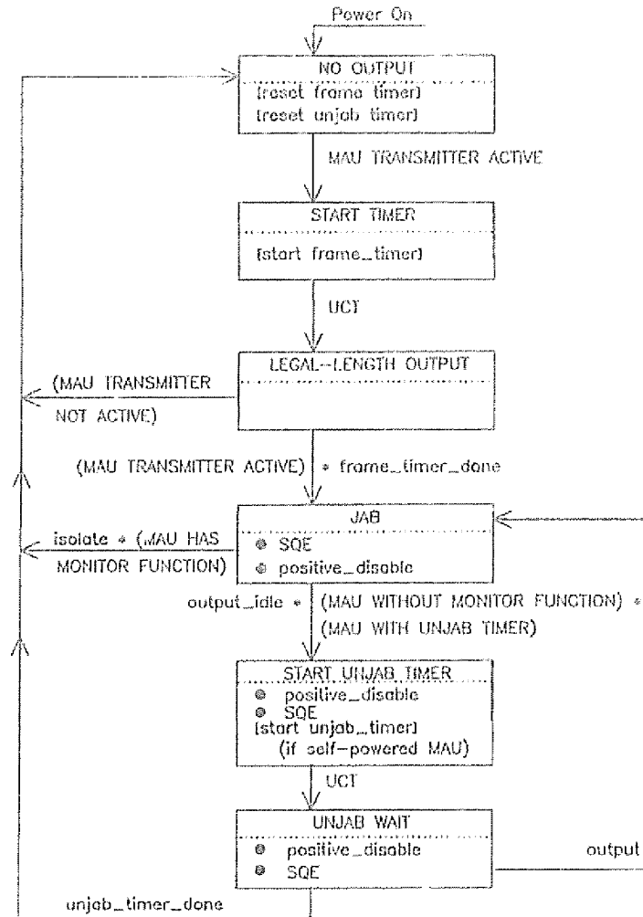
Fig 8.4 Jabber Function
