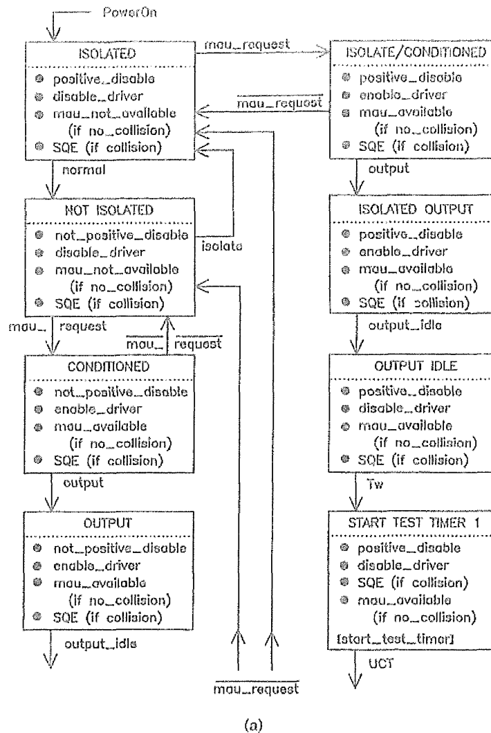
Fig 7-9 Interface Function for MAU with Conditioning
