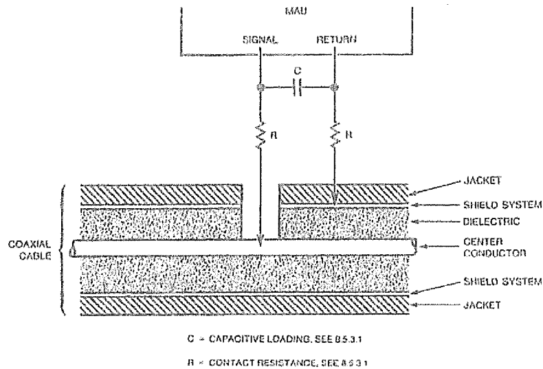
Fig 8-9 Typical Coaxial Tap Connection Circuit
