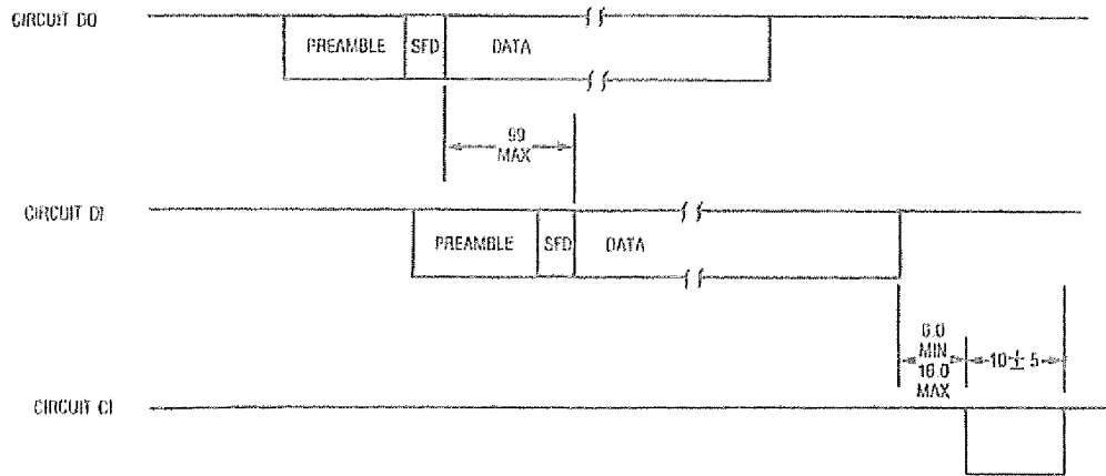
Fig 11-16 Timing at AUI for Zero-Length Coax
