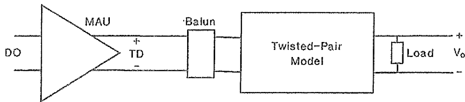
Fig 14-8 Differential Output Voltage Test
