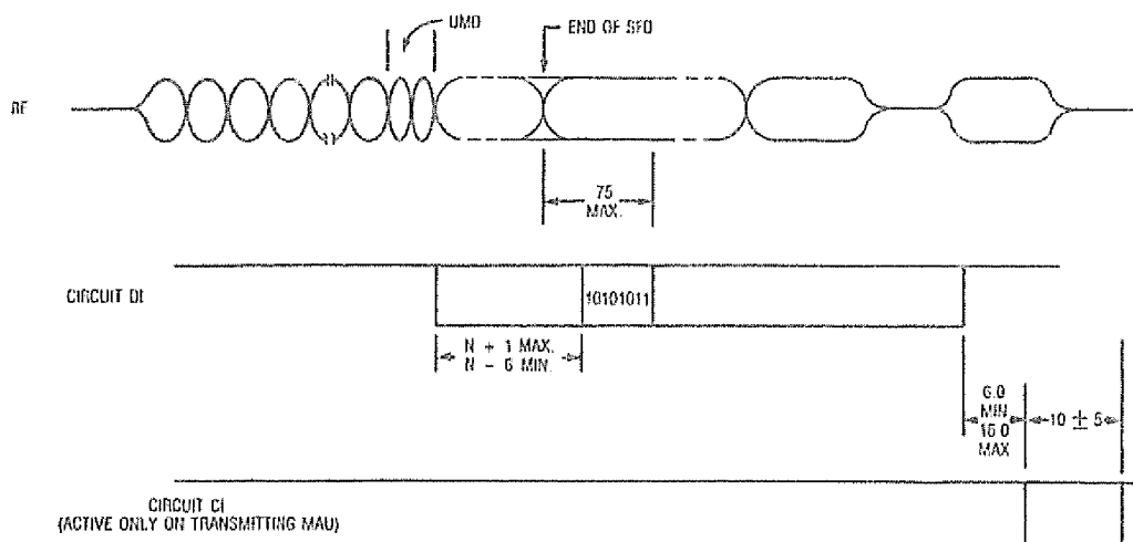
Fig 11-13 No Collision Timing Diagram (Coax to AUI)
