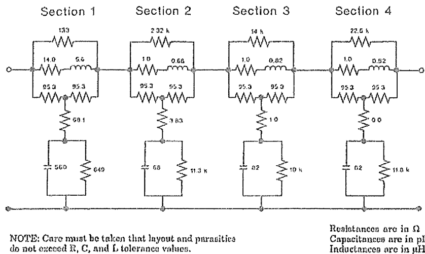
Fig 14-7 Twisted-Pair Model
