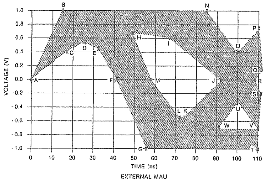
Fig 14-9 Voltage Template
