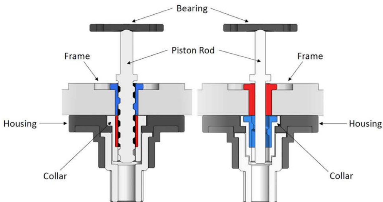
Cross-Sections of Collar Friction Model Configured to Demonstrate Steenfeldt-Jensen's Fifth Embodiment (left) and Petitioner's Proposed Modification (right)
