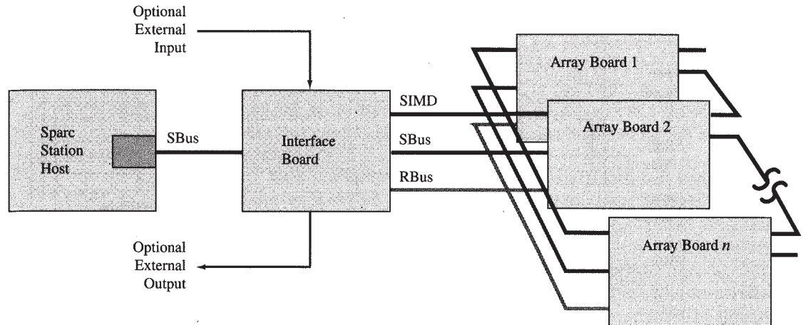
FIGURE 2.3 Splash 2 System Architecture
