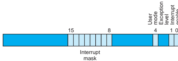
FIGURE A.7.1 The Status register.
