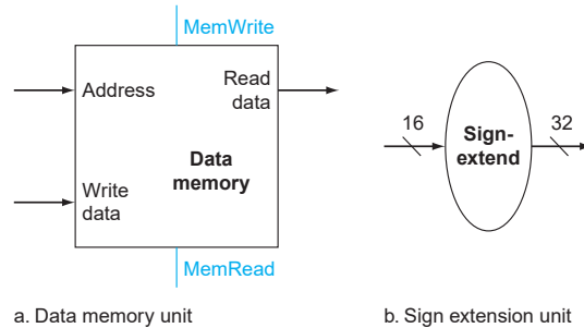
FIGURE 4.8 The two units needed to implement loads and stores, in addition to the register file and ALU of Figure 4.7, are the data memory unit and the sign extension unit.
