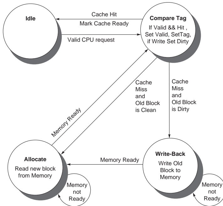
FIGURE 5.40 Four states of the simple controller.
