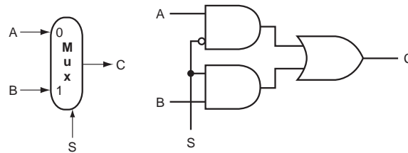
FIGURE B.3.2 A two-input multiplexer on the left and its implementation with gates on the right. The multiplexer has two data inputs ( A and B ), which are labeled 0 and 1 , and one selector input ( S ), as well as an output C . Implementing multiplexers in Verilog requires a little more work, especially when they are wider than two inputs. We show how to do this beginning on page B-23.
