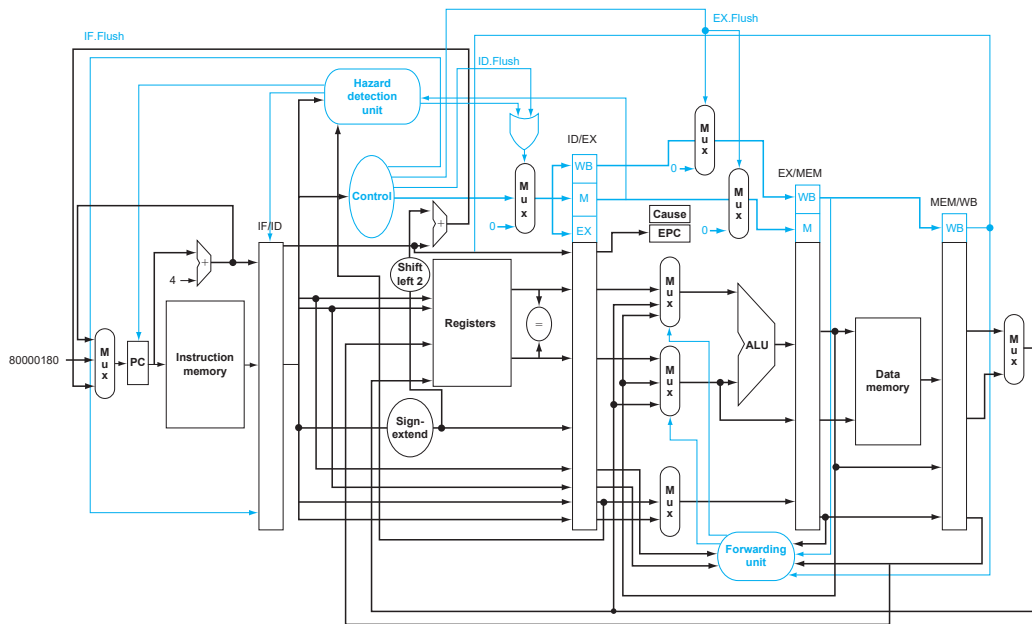
FIGURE 4.66 The datapath with controls to handle exceptions. The key additions include a new input with the value 8000\ 0180_{\text{hex}} in the multiplexer that supplies the new PC value; a Cause register to record the cause of the exception; and an Exception PC register to save the address of the instruction that caused the exception. The 8000\ 0180_{\text{hex}} input to the multiplexer is the initial address to begin fetching instructions in the event of an exception. Although not shown, the ALU overflow signal is an input to the control unit.
