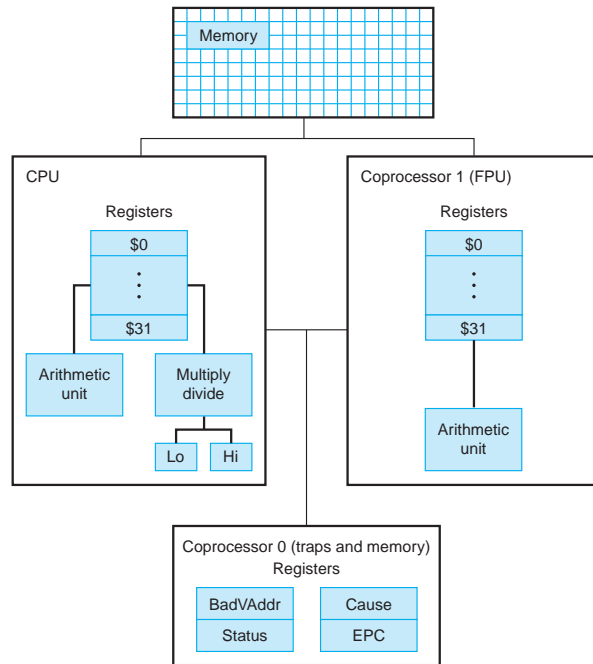
FIGURE A.10.1 MIPS R2000 CPU and FPU.
