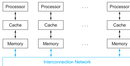
FIGURE 6.13 Classic organization of a multiprocessor with multiple private address spaces, traditionally called a message-passing multiprocessor . Note that unlike the SMP in Figure 6.7, the interconnection network is not between the caches and memory but is instead between processor-memory nodes.
