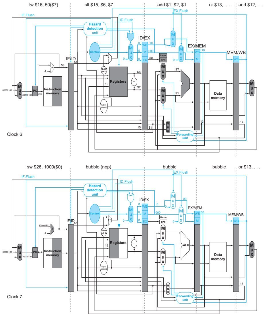
FIGURE 4.67 The result of an exception due to arithmetic overflow in the add instruction. The overflow is detected during the EX stage of clock 6, saving the address following the add in the EPC register ( 4C + 4 = 50_{hex} ). Overflow causes all the Flush signals to be set near the end of this clock cycle, deasserting control values (setting them to 0) for the add. Clock cycle 7 shows the instructions converted to bubbles in the pipeline plus the fetching of the first instruction of the exception routine— sw $25, 1000($0) —from instruction location 8000\ 0180_{hex} . Note that the AND and OR instructions, which are prior to the add, still complete. Although not shown, the ALU overflow signal is an input to the control unit.
